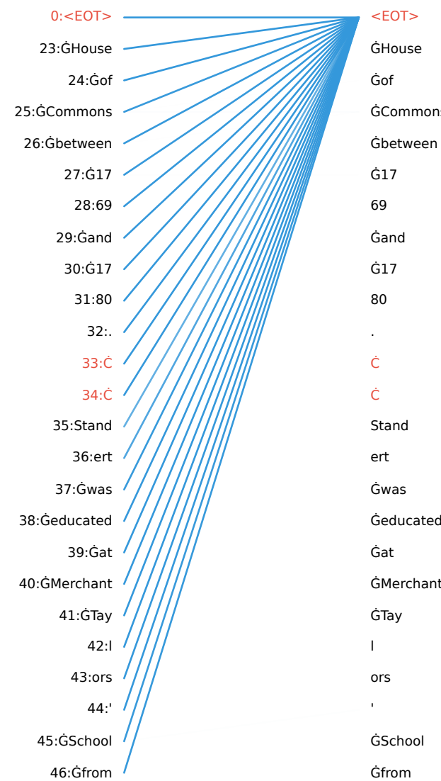
L08H03: initial-key sink shown-key mass=0.98
