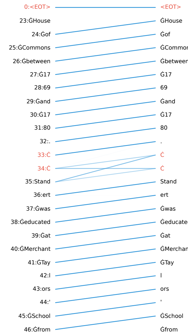
L05H12: previous-token attention shown-key mass=0.96
