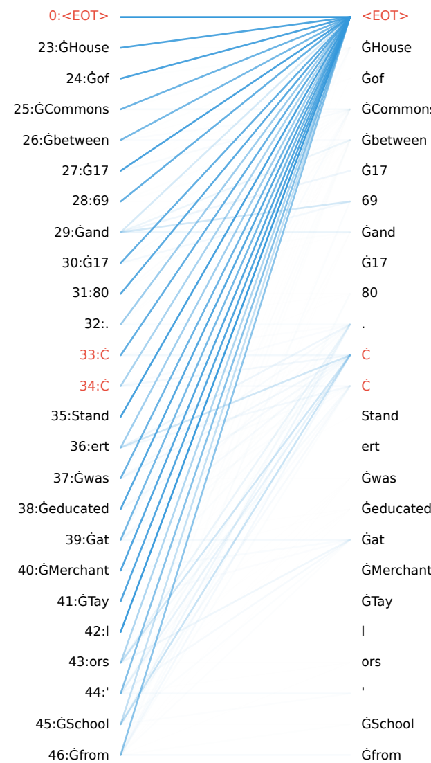
L11H04: boundary candidate shown-key mass=0.84
