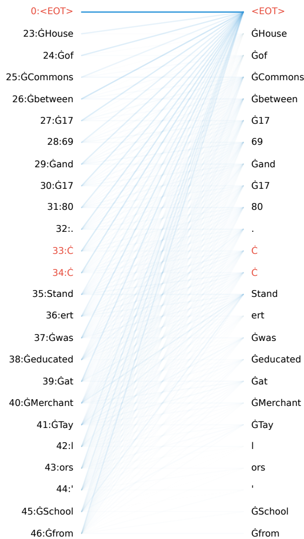
L01H12: broad attention shown-key mass=0.40
