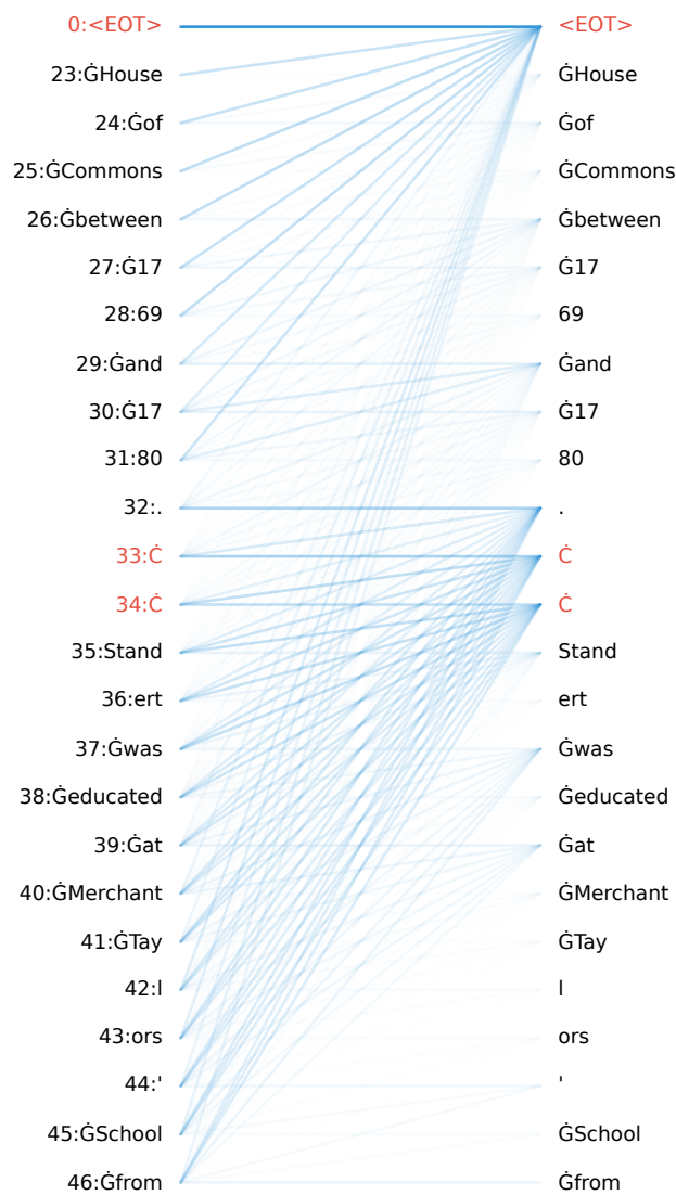
L03H07: periods/newlines shown-key mass=0.73
