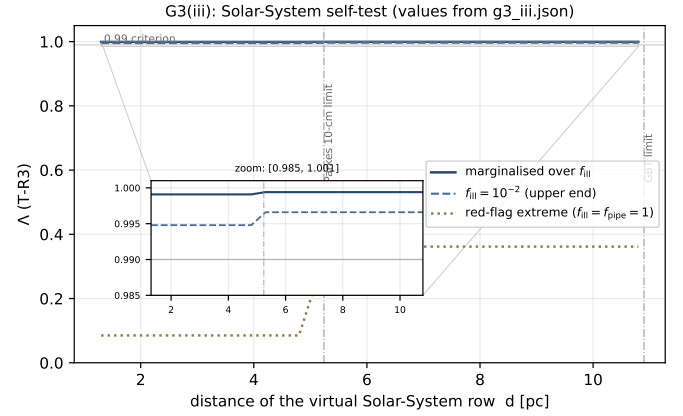
Fig. 1. The G3(iii) Solar-System self-test as d – \Lambda . Three curves (marginalised; f_{ill} = 10^{-2} , the upper end; the extreme f_{ill} = f_{pipe} = 1 ) with the sensitivity boundaries (Parkes 5.24 pc, GBT 10.9 pc). Values are the frozen g3_iii.json . Reproduce: python3 scripts/build_paper_figs.py
