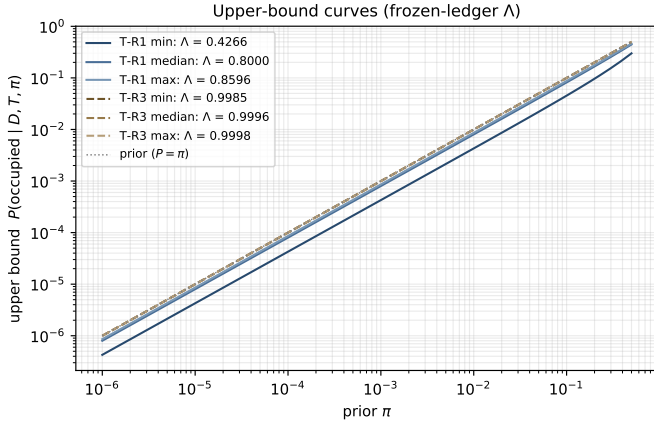
Fig. 4. Upper-bound curves P(\text{occupied} \mid D, T, \pi) = \text{expit}(\text{logit } \pi + \ln \Lambda) . Curves use the frozen-ledger \Lambda (min/median/max of T-R1 and T-R3); the dotted line is the prior P = \pi . Reproduce: python3 scripts/build_paper_figs.py
