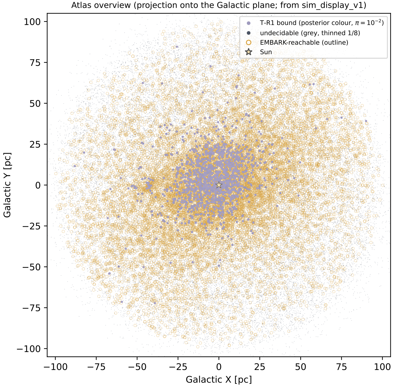
Fig. 3. Atlas overview (projection onto the Galactic plane, machine-generated from sim_display_v1 ). Undecidable stars in grey (thinned 1/8); stars with a T-R1 bound in the value-neutral continuous colour of the posterior at \pi = 10^{-2} ; EMBARK-reachable stars as outlines; the Sun as a star marker. Same colour discipline as the simulator. Reproduce: python3 scripts/build_paper_figs.py
