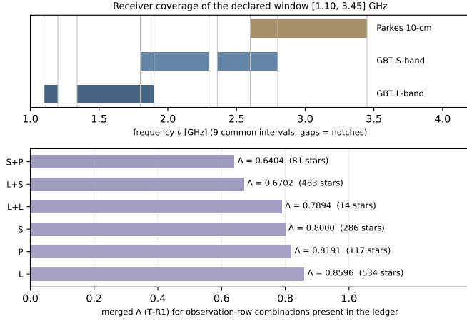
Fig. 2. Receiver coverage of the declared window [1.10, 3.45] GHz (top: the 9 common intervals and notches) and the merged \Lambda for the six most frequent observation-row combinations present in the ledger (bottom: T-R1; 1,515 stars in total, the remaining 39 stars being rarer combinations of three or more rows; bar colours follow the posterior colour rule at \pi = 10^{-2} ). Values are the frozen radio_obs_v0.json and lambda_ledger.json . Reproduce: python3 scripts/build_paper_figs.py
