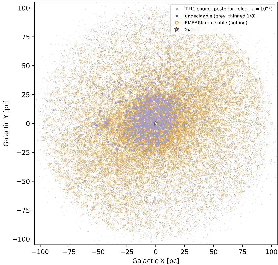
Atlas overview (projection onto the Galactic plane; from sim_display_v1)
