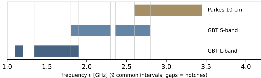
Receiver coverage of the declared window [1.10, 3.45] GHz
