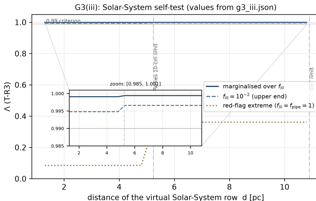
図 1: G3(iii) 太陽系自己検定の d - \Lambda 。周辺化値・ f_{\text{III}} = 10^{-2} (上端)・極限 ( f_{\text{III}} = f_{\text{pipe}} = 1 ) の 3 曲線と感度境界 (Parkes 5.24 pc、GBT 10.9 pc)。数値は g3_iii.json の凍結値。再現: python3 scripts/build_paper_figs.py
