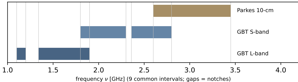
Receiver coverage of the declared window [1.10, 3.45] GHz
