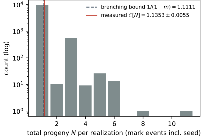
Figure 1: Reverse channel (experiment E8c): histogram of the total progeny N (mark events including the seed) over 10^4 realizations in the counterexample regime. The measured mean exceeds the branching bound by 4.4\sigma . Reproduce: python3 src/wake_r/paper_figs.py (data: data/phase_r/E8c_counterexample.json ).
