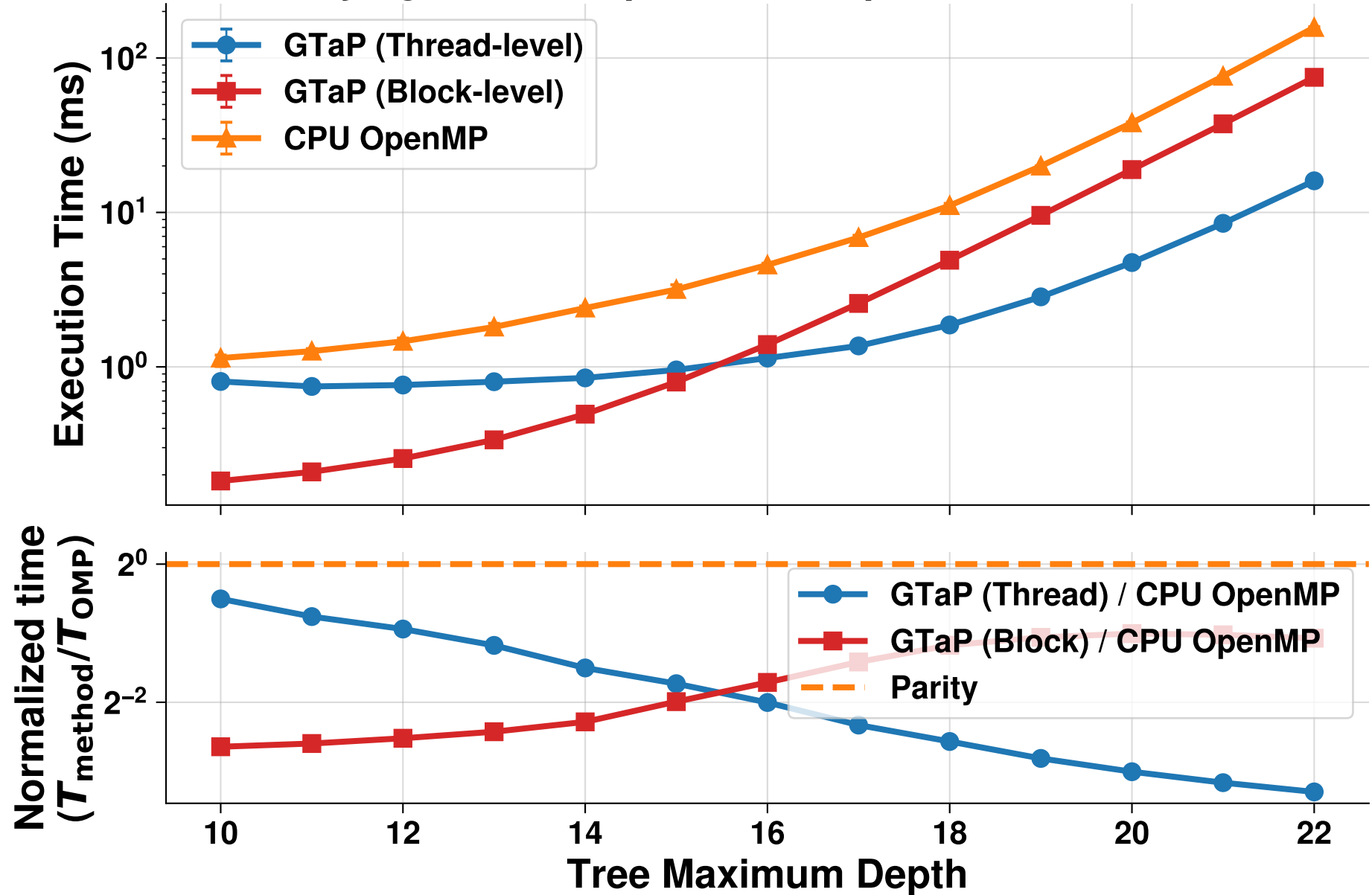
Varying D (mem_ops=256, compute_iters=256 fixed)
