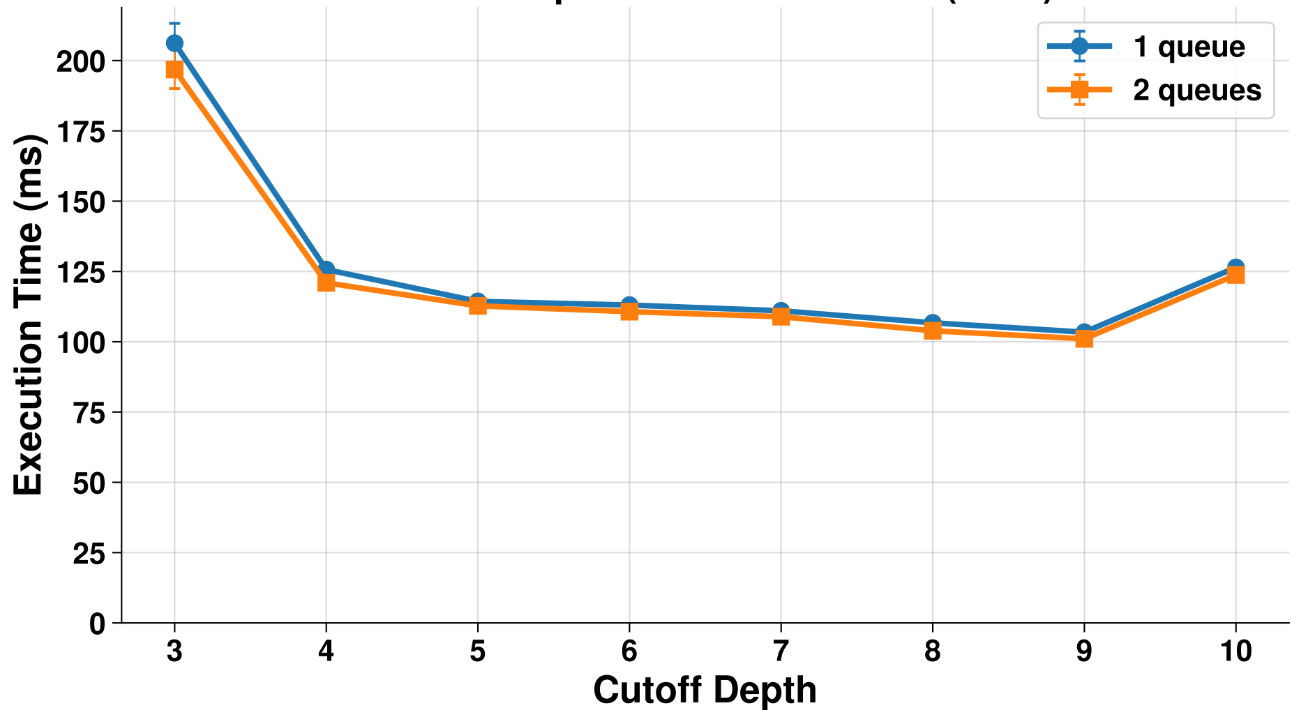
EPAQ Comparison for N-Queens (n=16)
