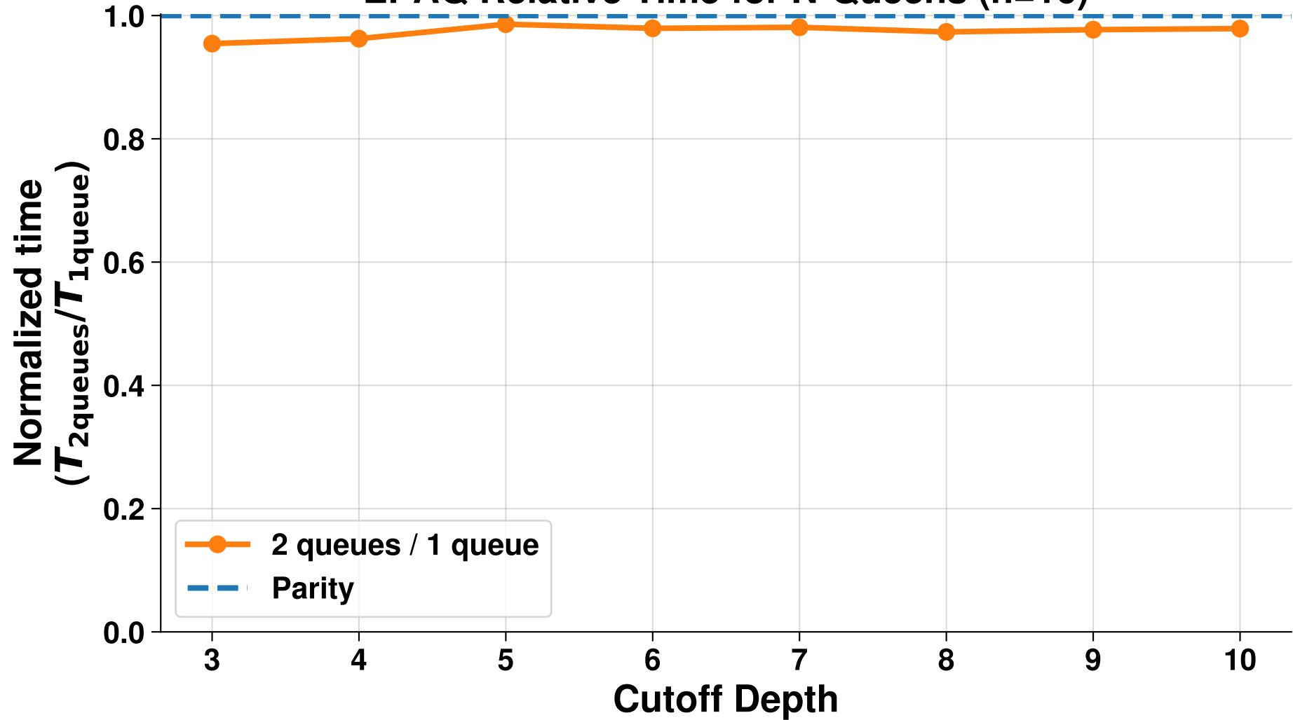
EPAQ Relative Time for N-Queens (n=16)
