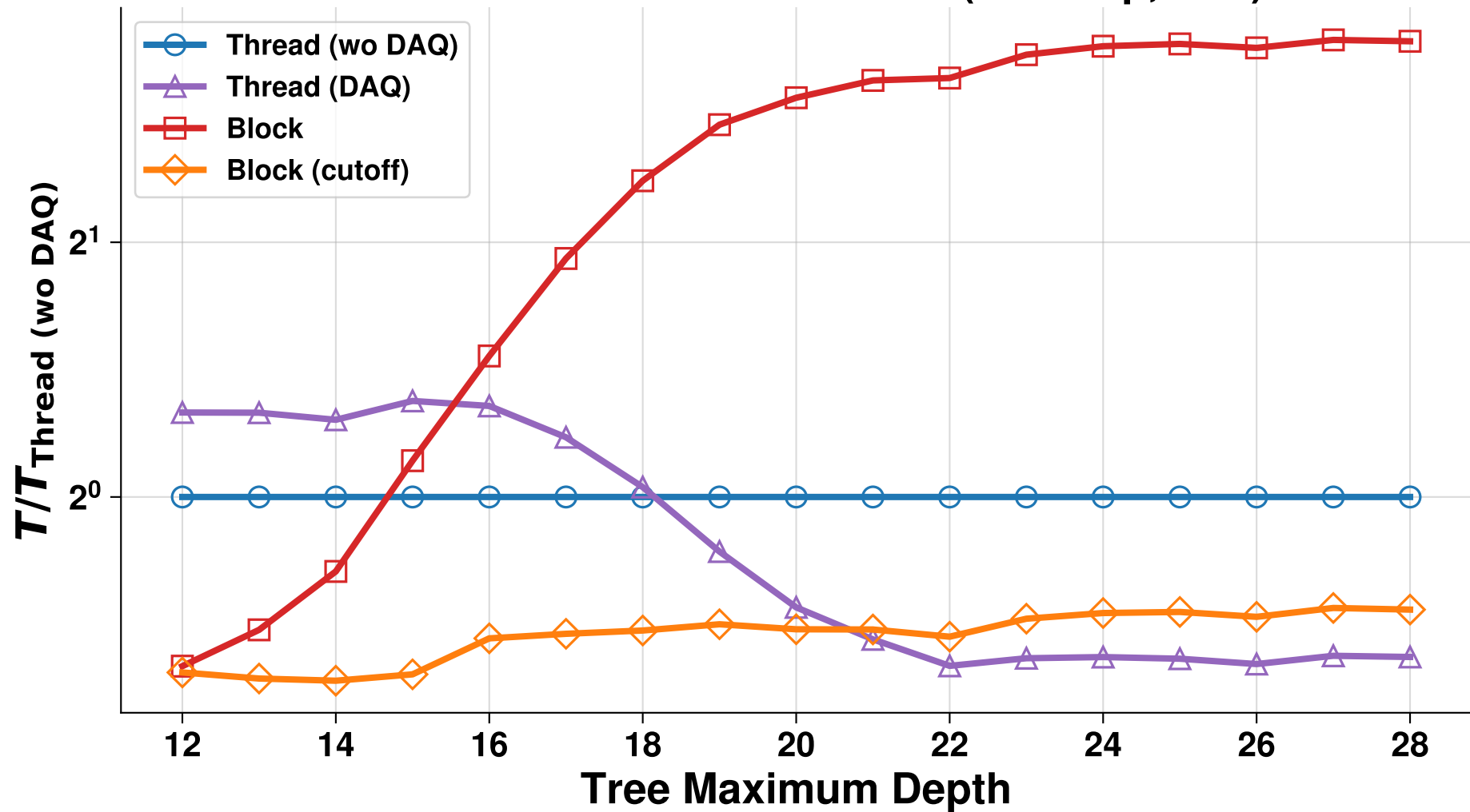
Normalized vs Thread wo DAQ (D sweep, K=2)
