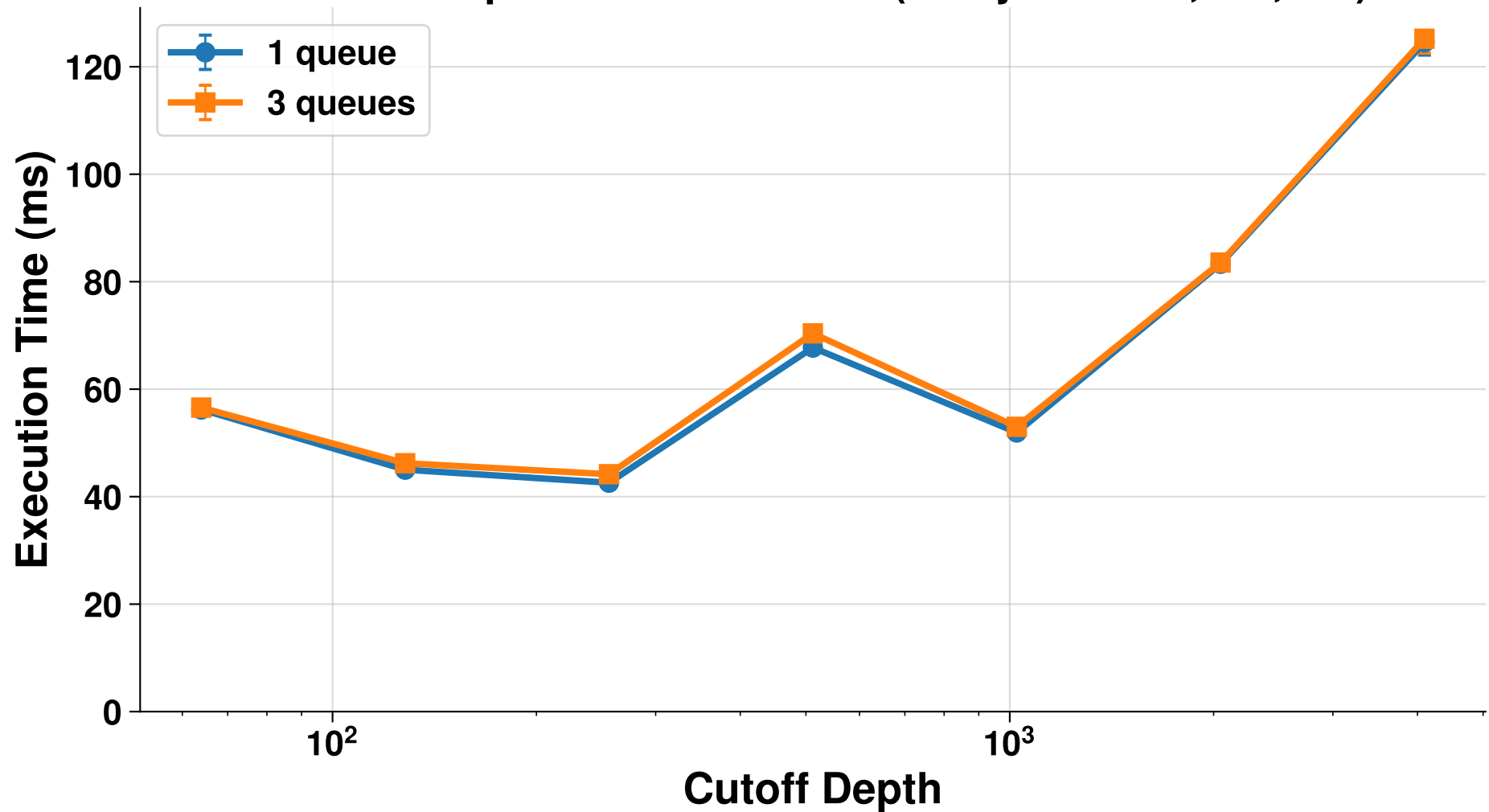
EPAQ Comparison for Cilkstart (Array Size=50,000,000)
