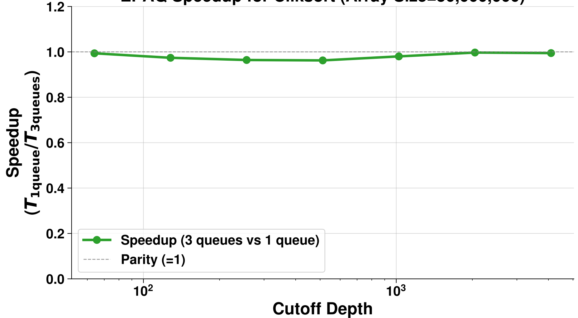
EPAQ Speedup for Cilksort (Array Size=50,000,000)
