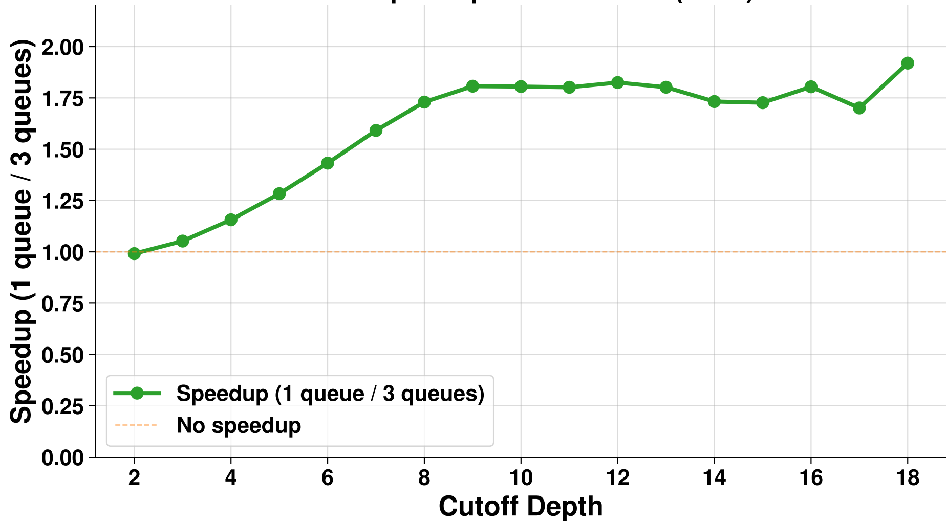
EPAQ Speedup for Fibonacci (n=40)
