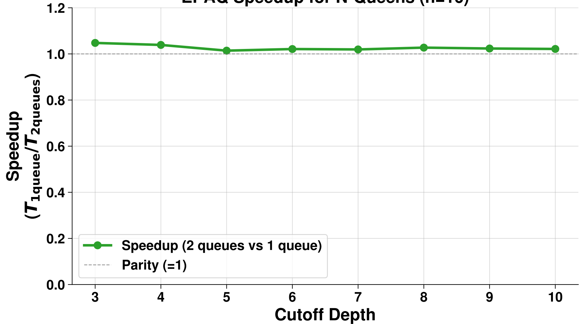
EPAQ Speedup for N-Queens (n=16)
