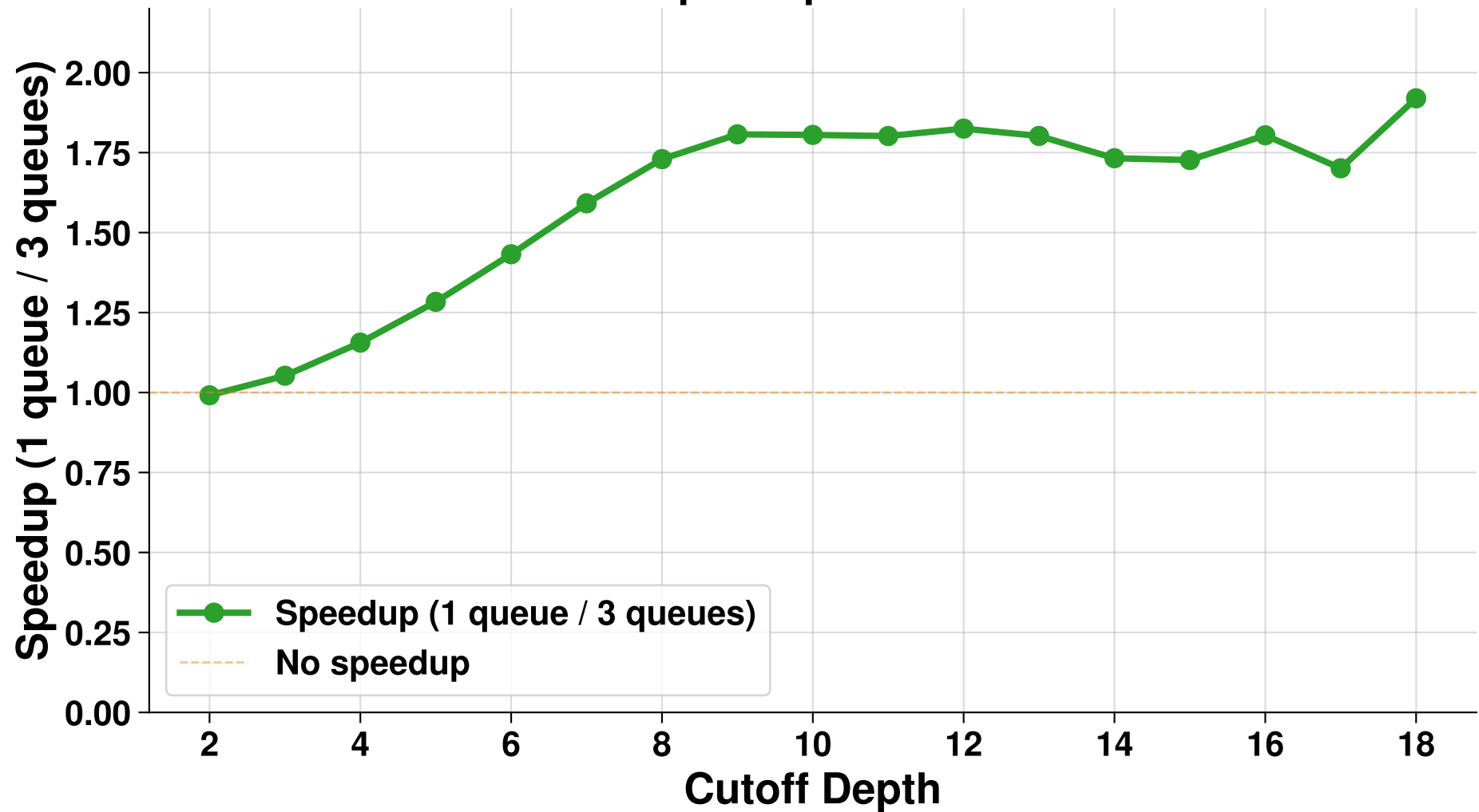
EPAQ Speedup for Fibonacci
