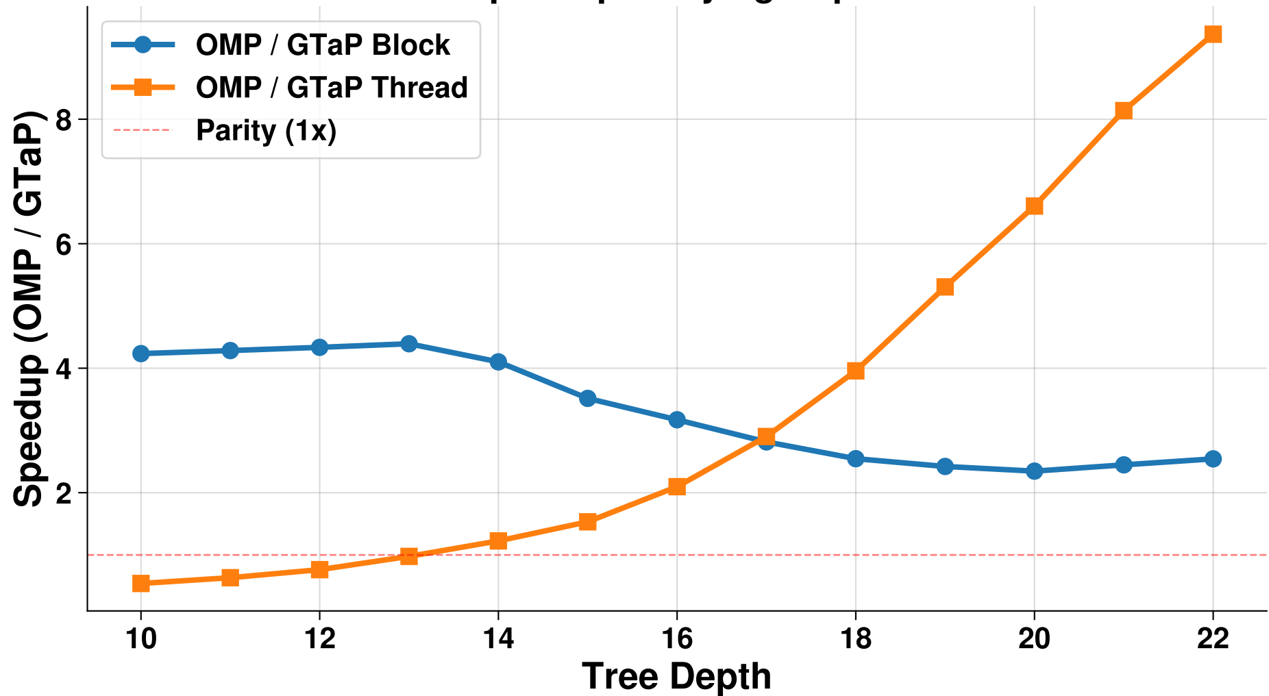
Speedup: Varying Depth
