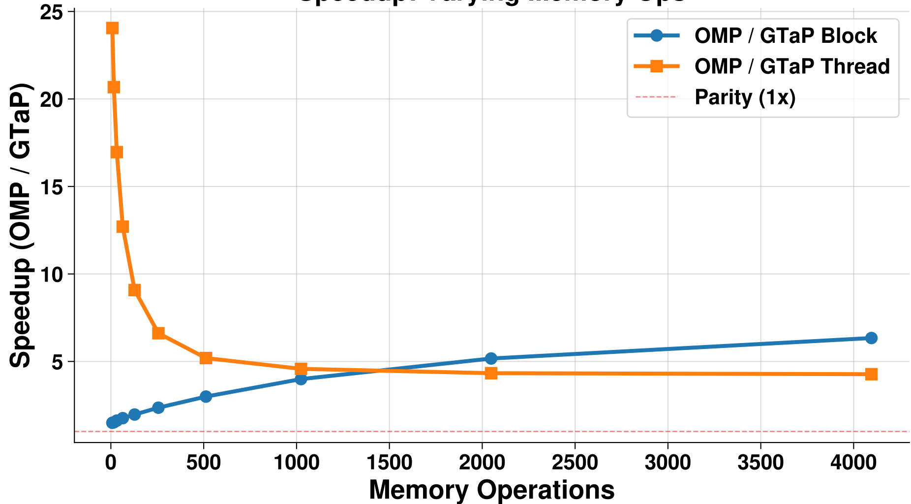
Speedup: Varying Memory Ops
