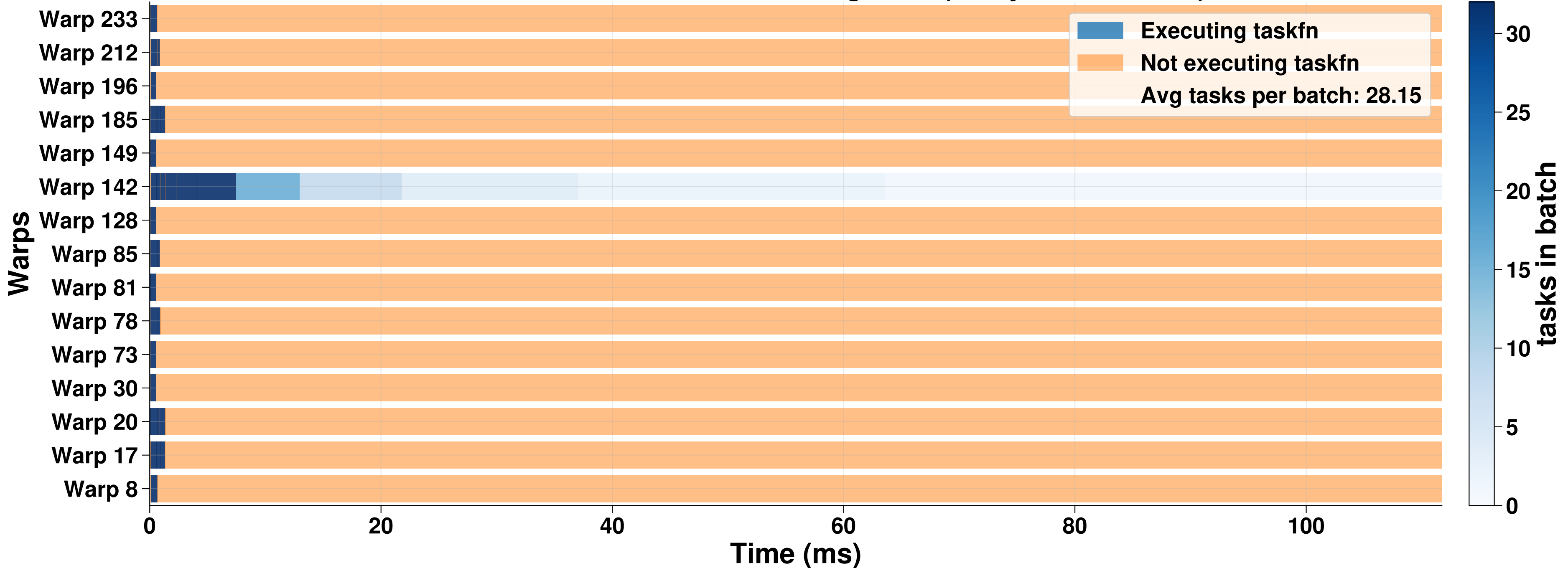
Worker Timeline Visualization: MergeSort (Array Size=2×10^5)
