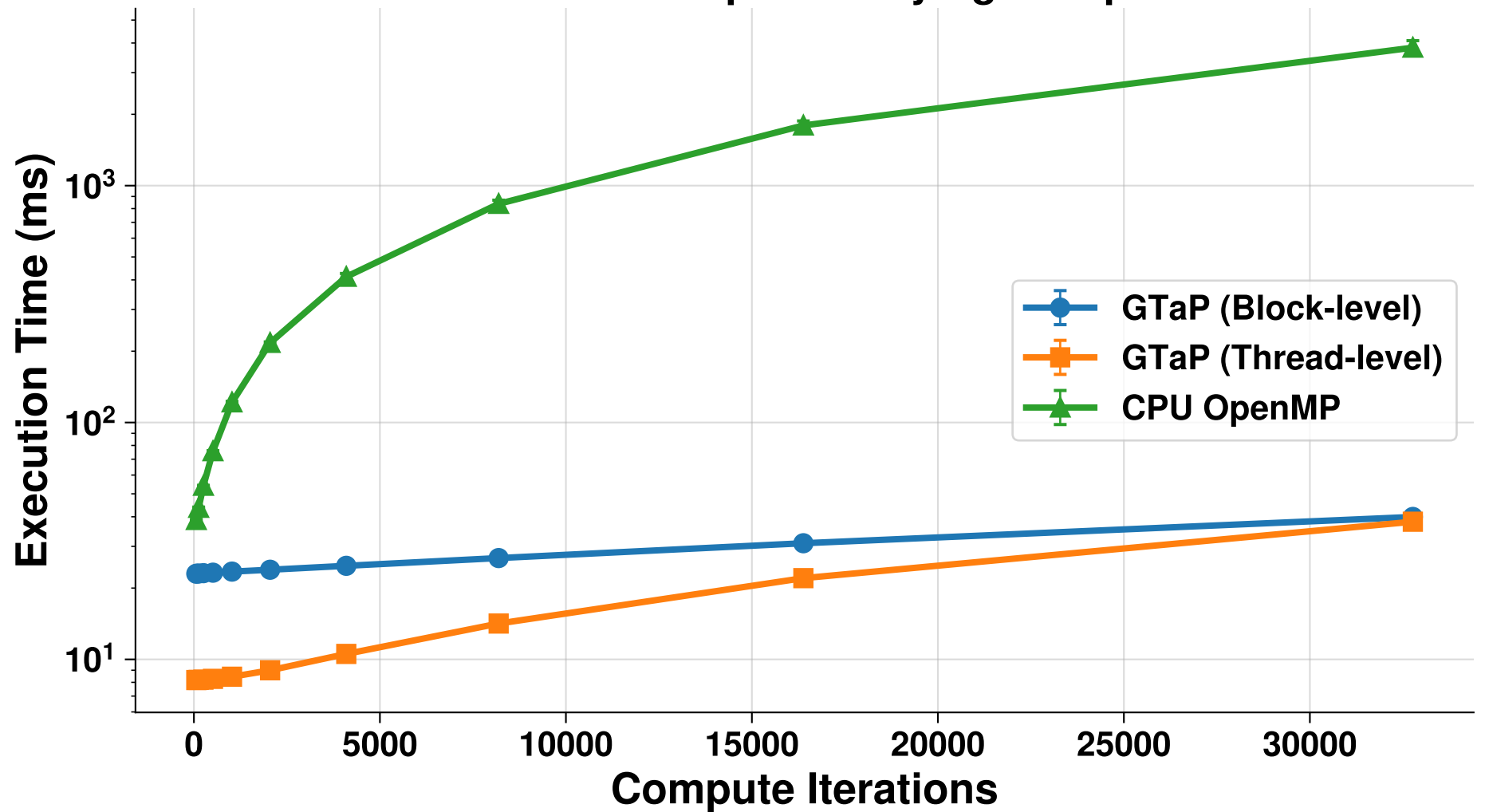
Tree Load/Compute: Varying Compute
