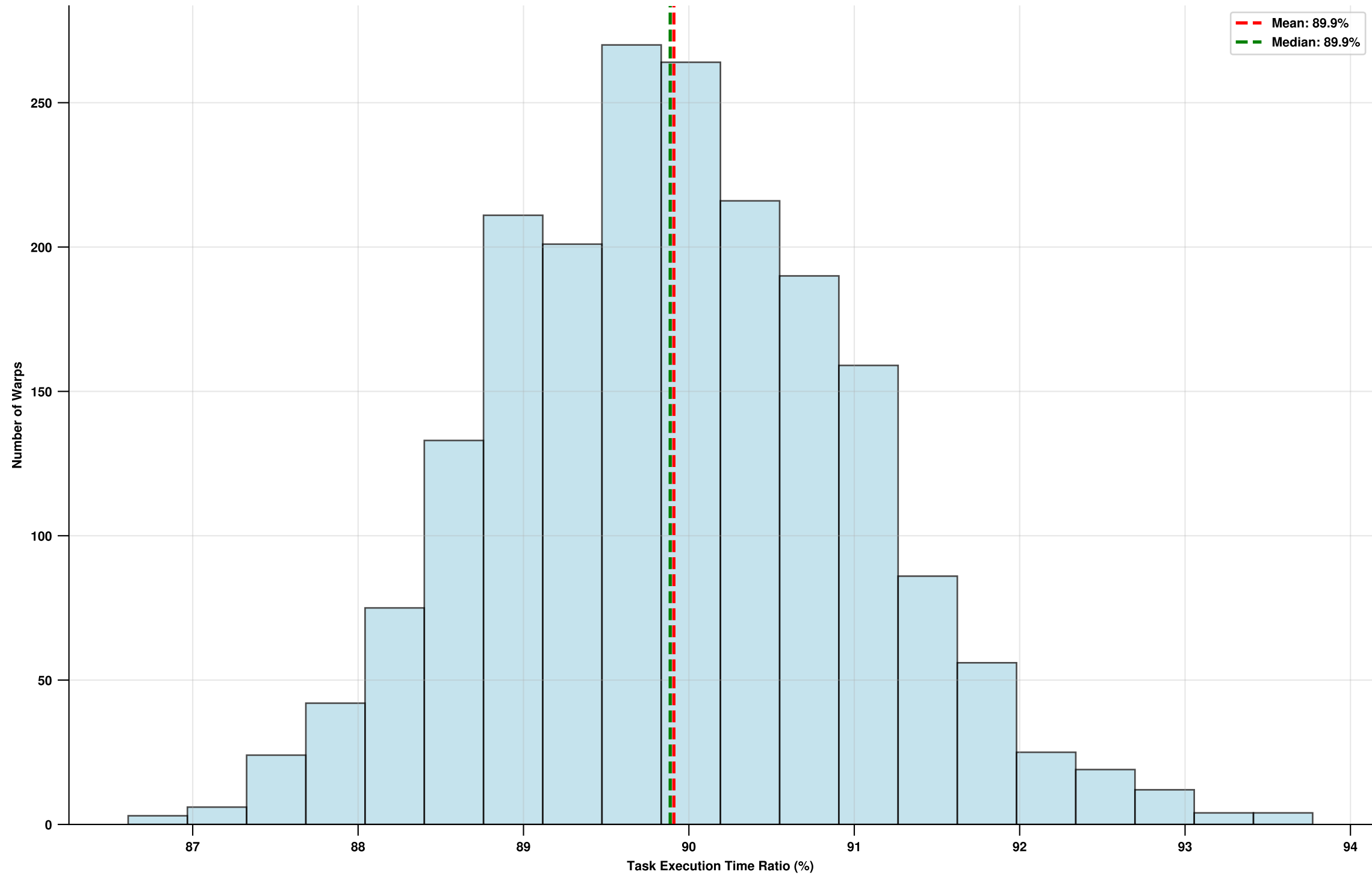
Distribution of Task Execution Time Ratio per Warp: Full Binary Tree
