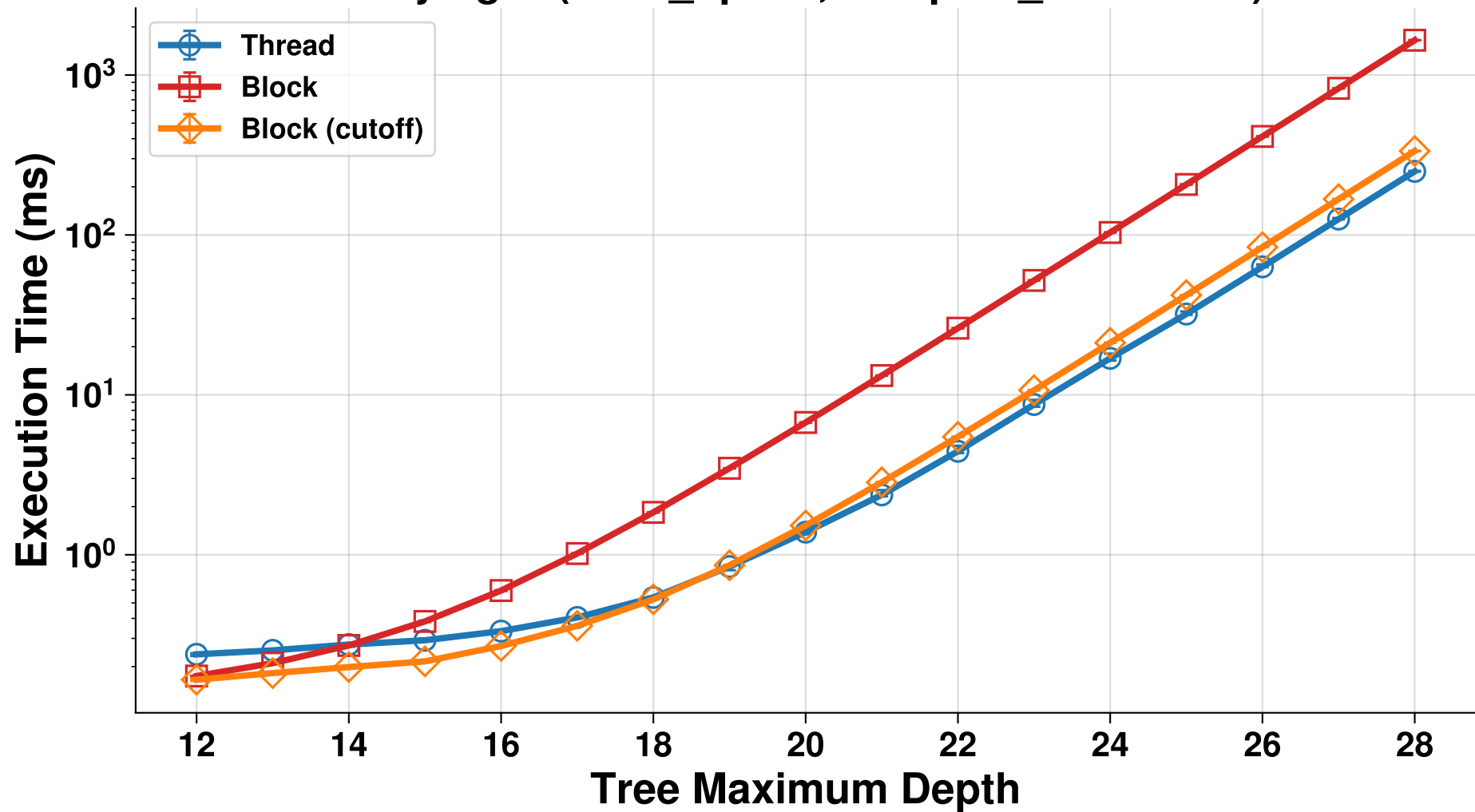
Varying D (mem_ops=0, compute_iters=2048)
