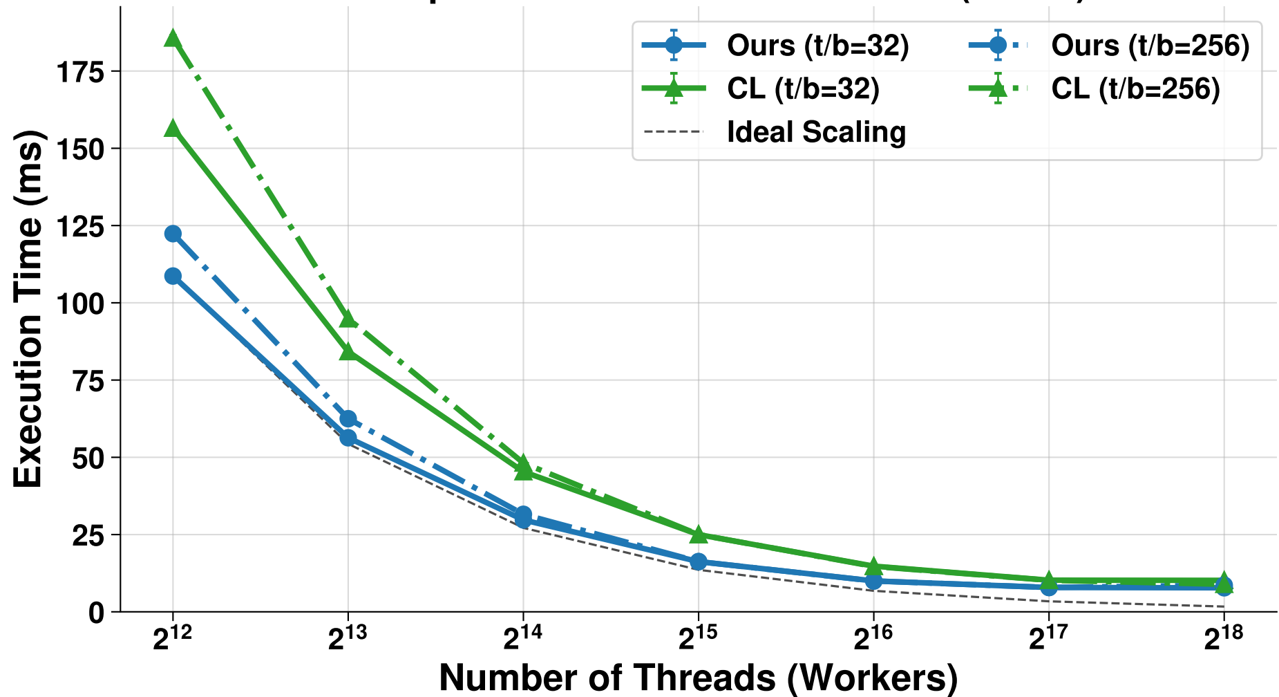
vs. Sequential Chase-Lev: Fibonacci (n = 35)
