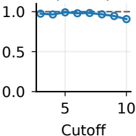
N-Queens ( n = 16 )
