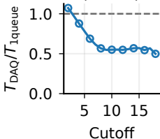
Fibonacci ( n = 40 )
