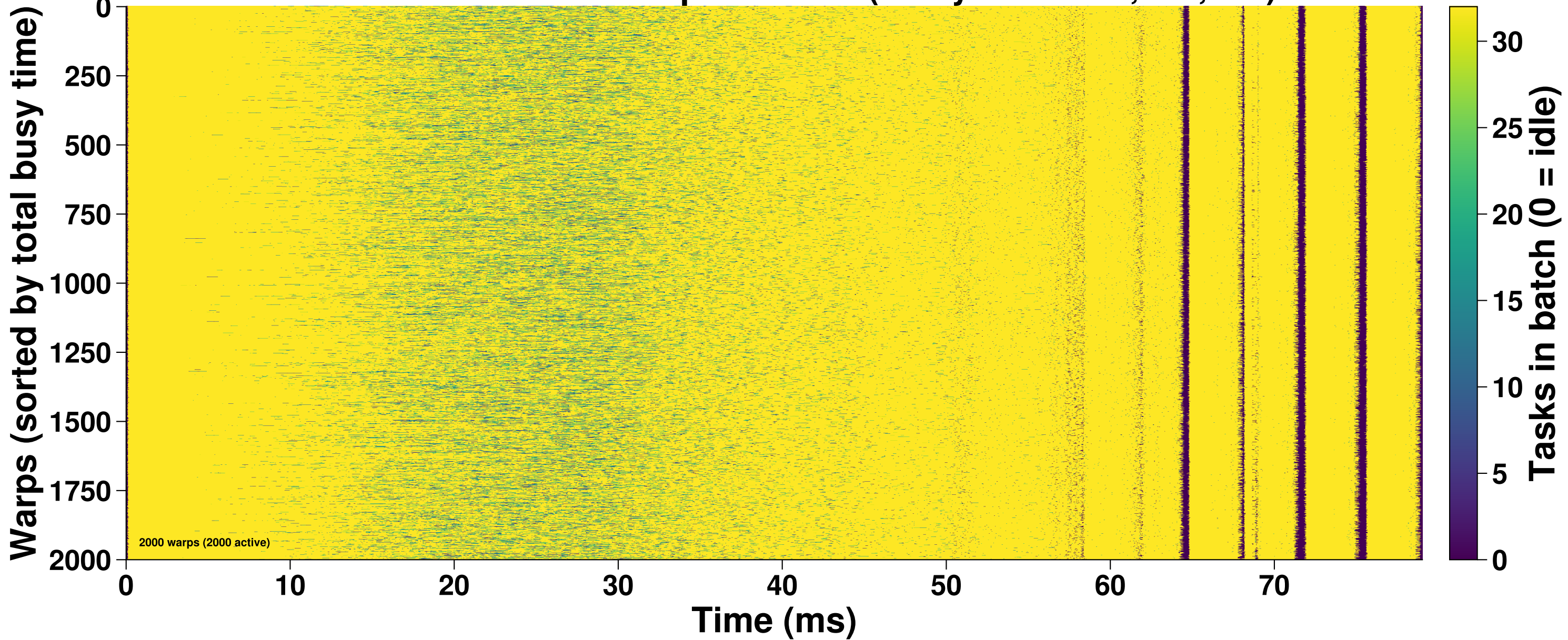
Worker Timeline Heatmap: CilkSort (Array Size=100,000,000)
