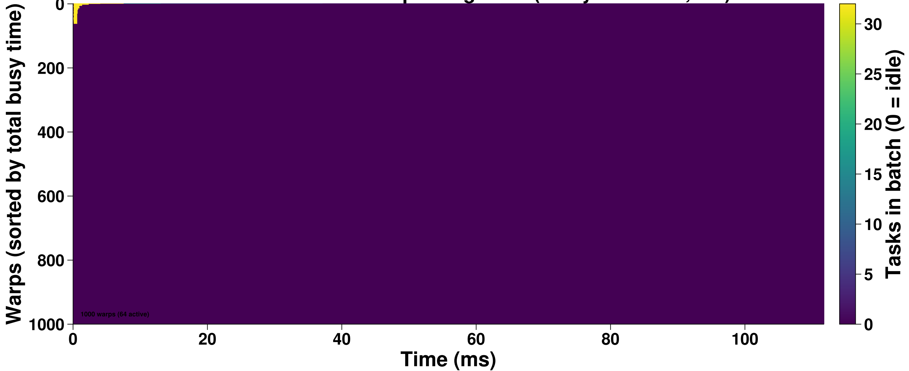
Worker Timeline Heatmap: MergeSort (Array Size=200,000)
