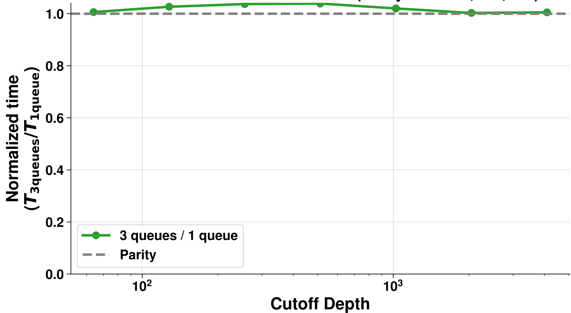
EPAQ Relative Time for CilkSORT (Array Size=50,000,000)
