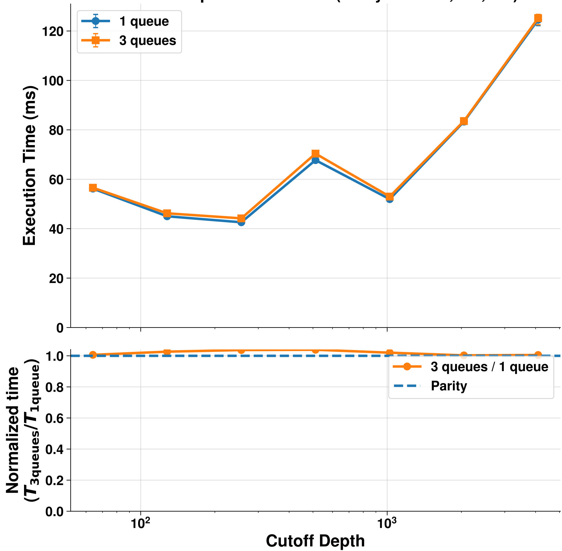
EPAQ Comparison: CilkSORT (Array Size=50,000,000)
