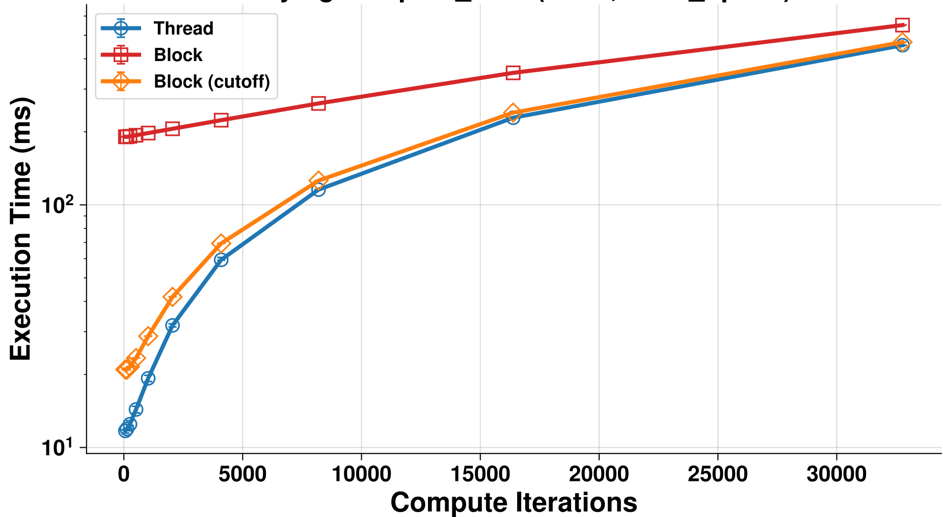
Varying compute_iters (D=25, mem_ops=0)
