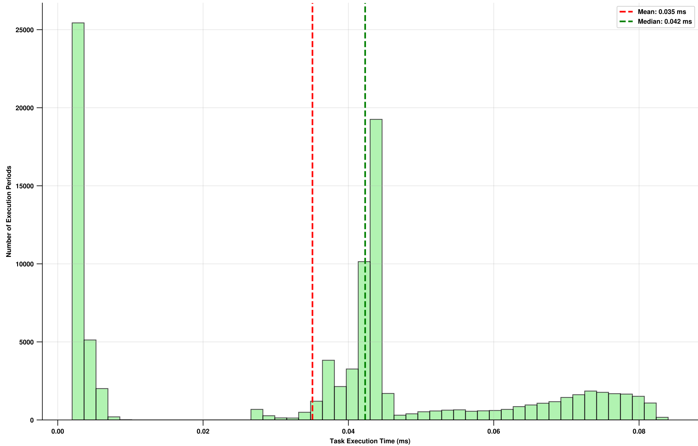
Distribution of Task Execution Time per Loop: Full Binary Tree (Thread-level workers)
