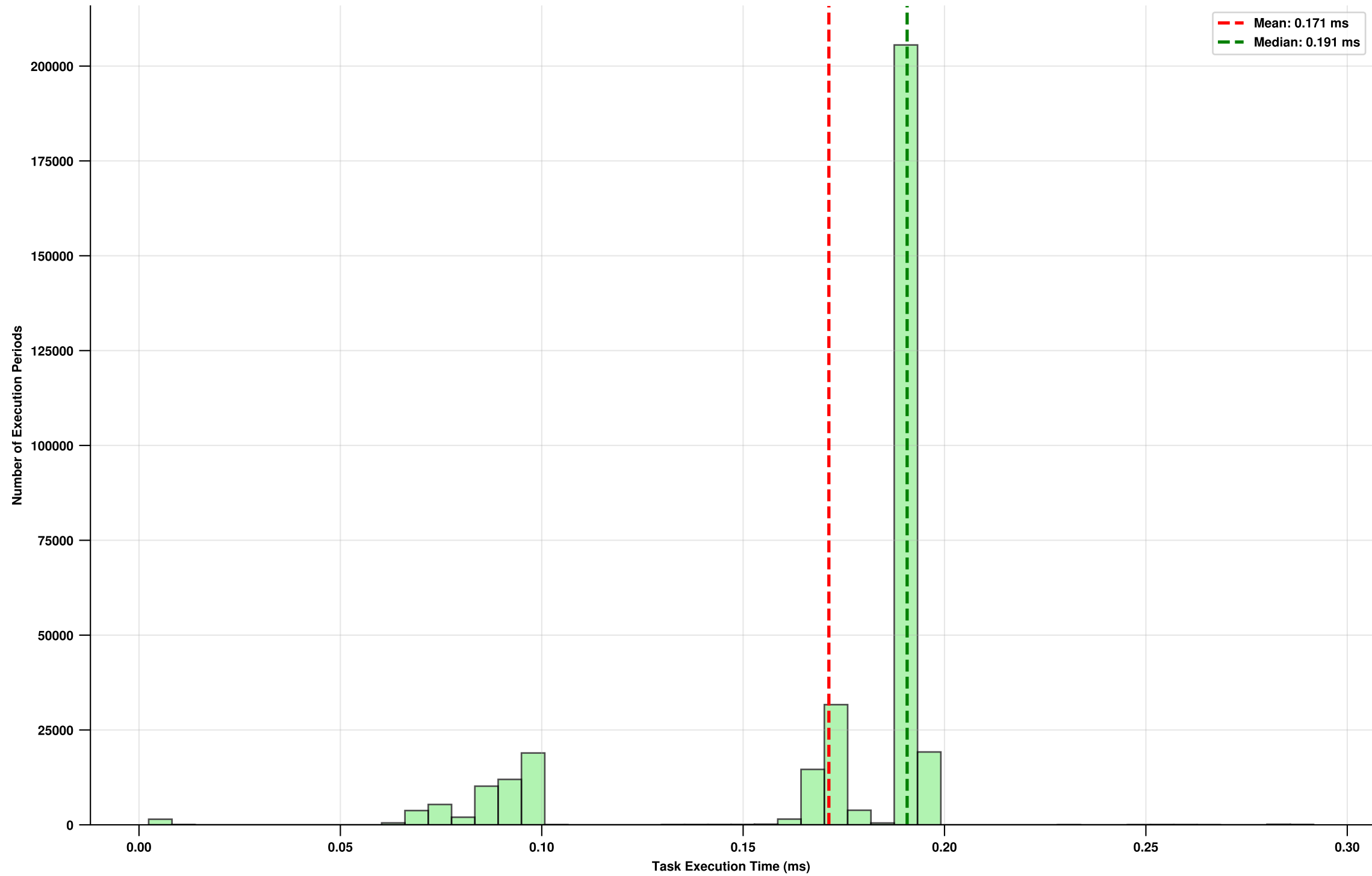
Distribution of Task Execution Time per Loop: Pruned B-ary Tree (Thread-level workers)
