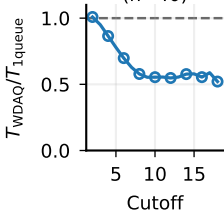
Fibonacci ( n=40 )
