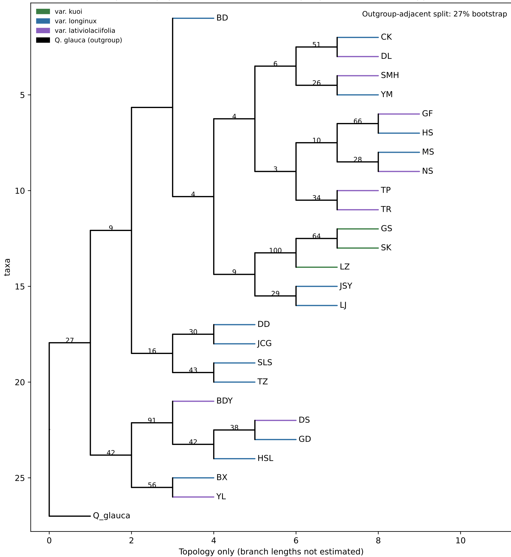
SVDquartets population tree (100 bootstrap replicates; all node supports)
