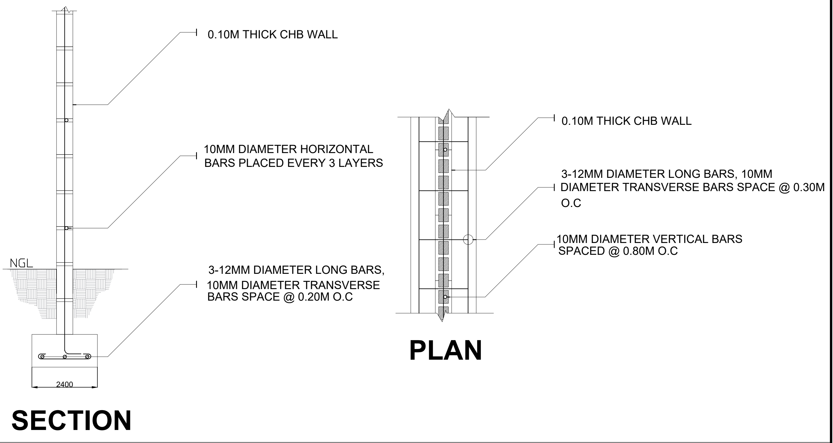
DETAILS OF W1F1 SCALE 1:100 MTRS.
