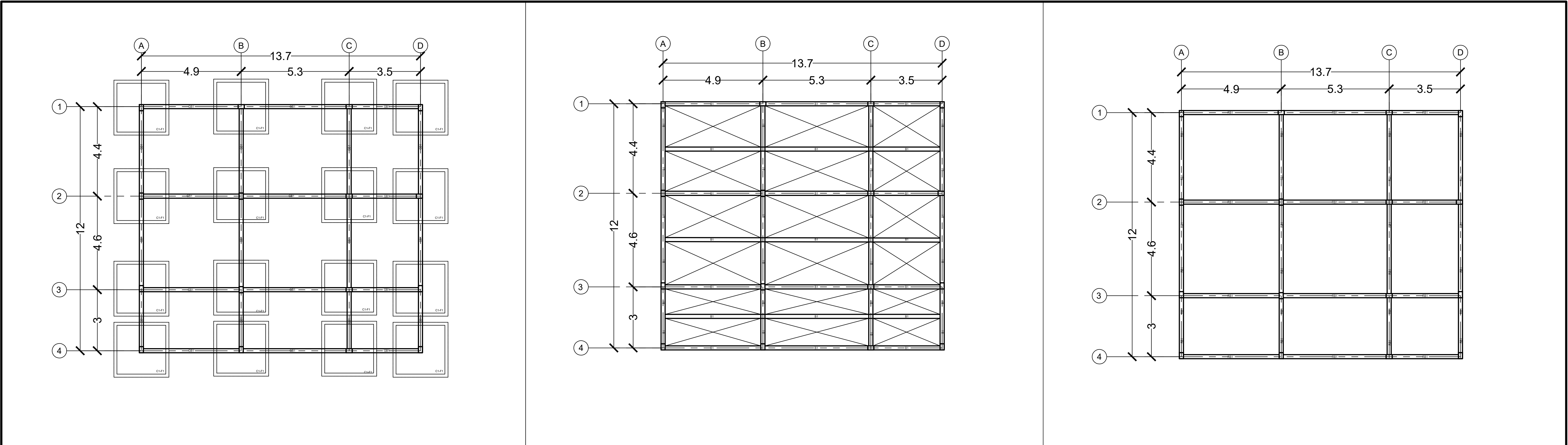
FOUNDATION PLAN SCALE 1:100 MTRS.
