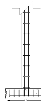
COLUMN FOOTING DETAIL 1:50 MTS
