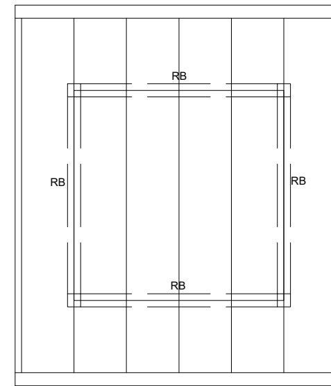
ROOF FRAMING PLAN 1:100 MTS
