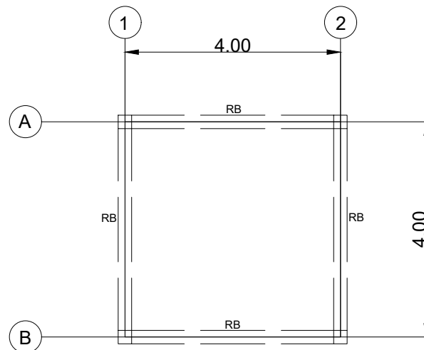
ROOF BEAM PLAN 1:100 MTS
