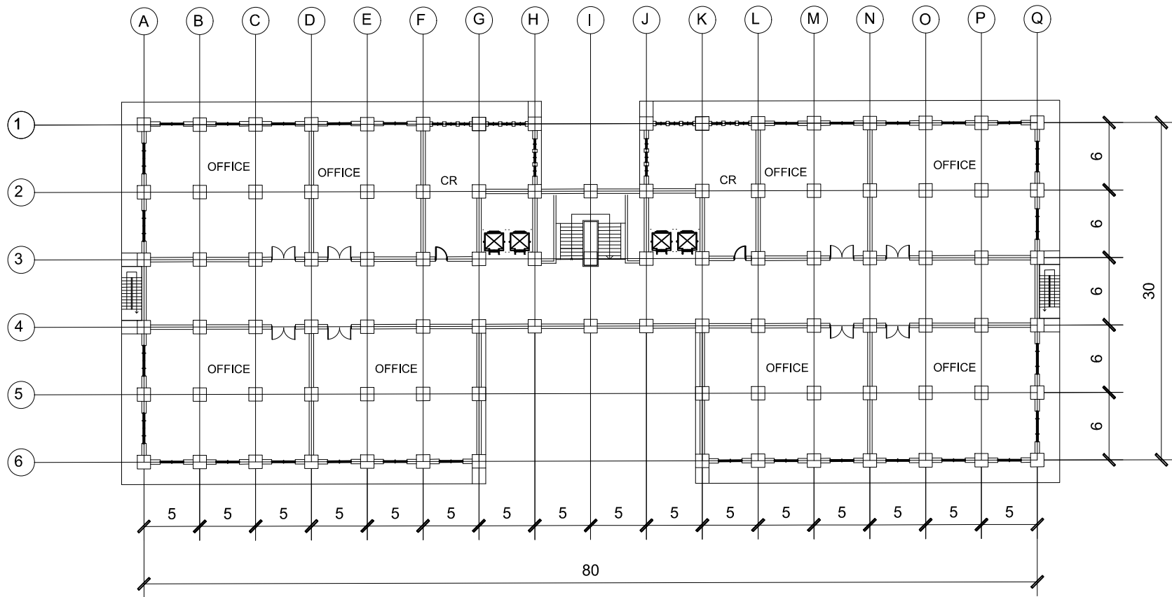
FOURTH FLOOR PLAN 1:100
