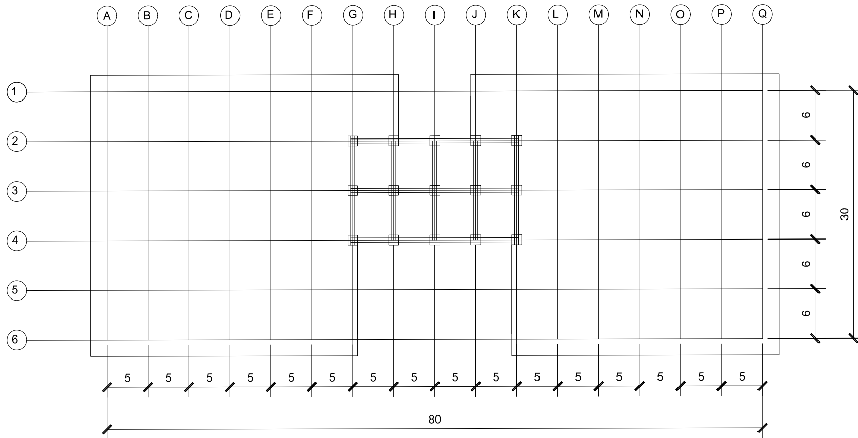
ROOF DECK STRUCTURAL FRAME
