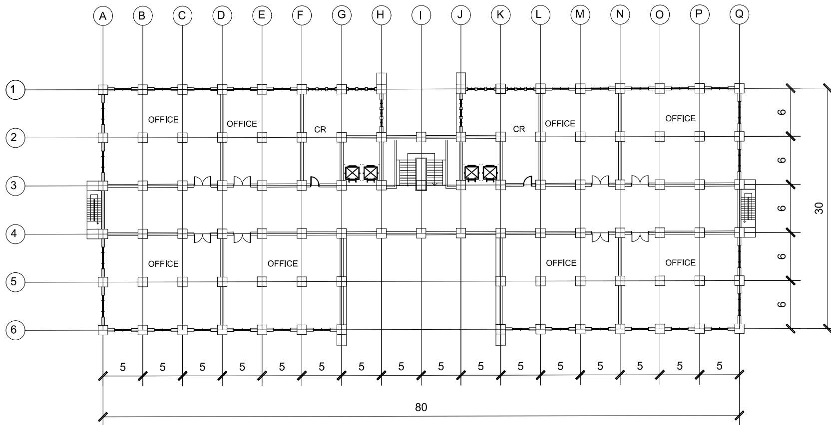
FIFTH FLOOR PLAN 1:100
