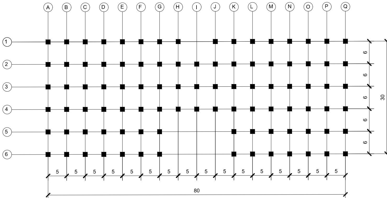
COLUMN LAYOUT AND SCHEDULE 1:100
