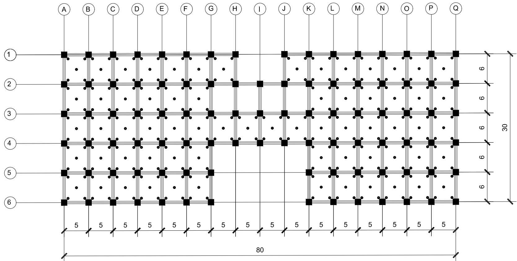
SECOND FLOOR CEILING PLAN
