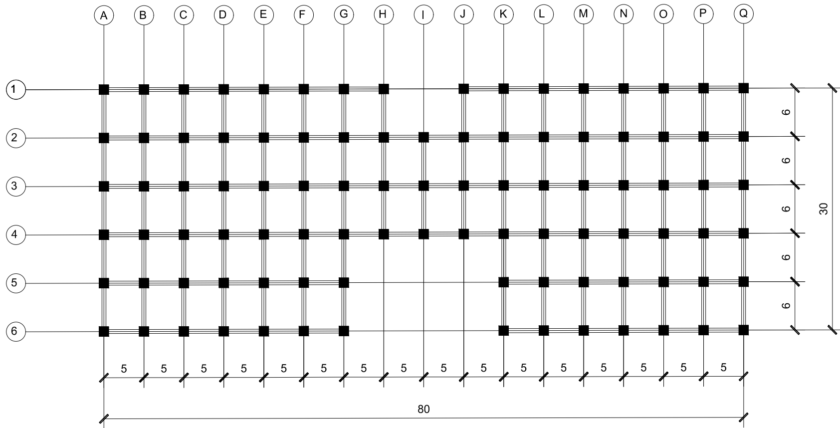
THIRD FLOOR STRUCTURAL FRAME
