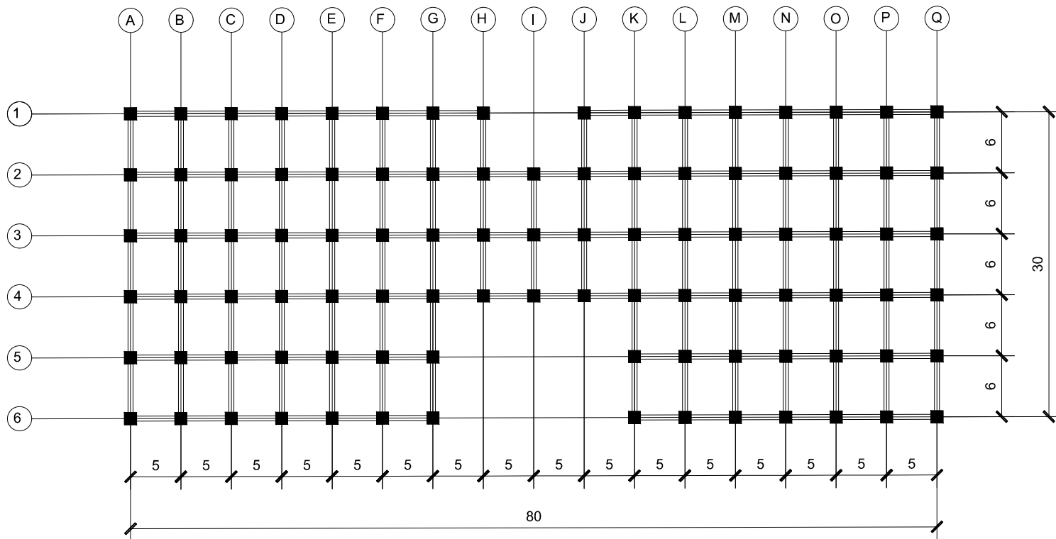
BEAM LAYOUT AND SCHEDULE 1:100
