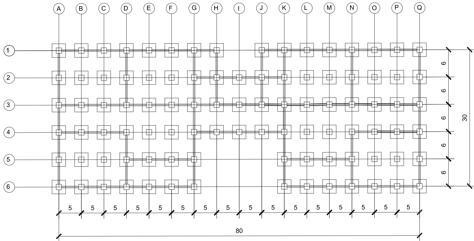
FOUNDATION PLAN
