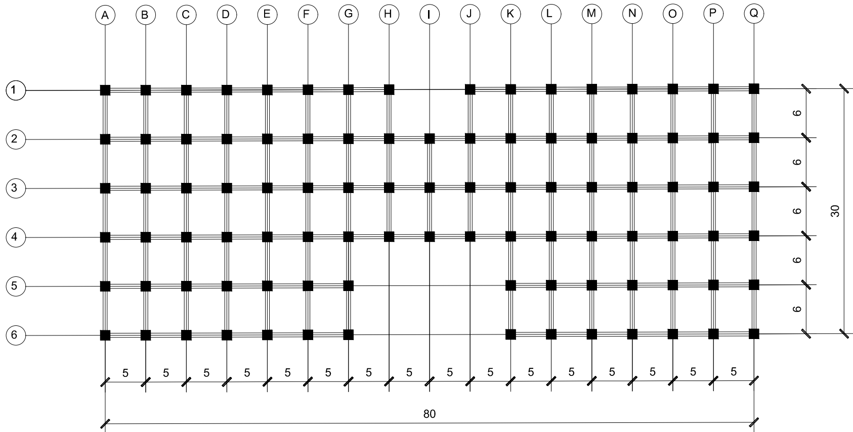
FOURTH FLOOR STRUCTURAL FRAME
