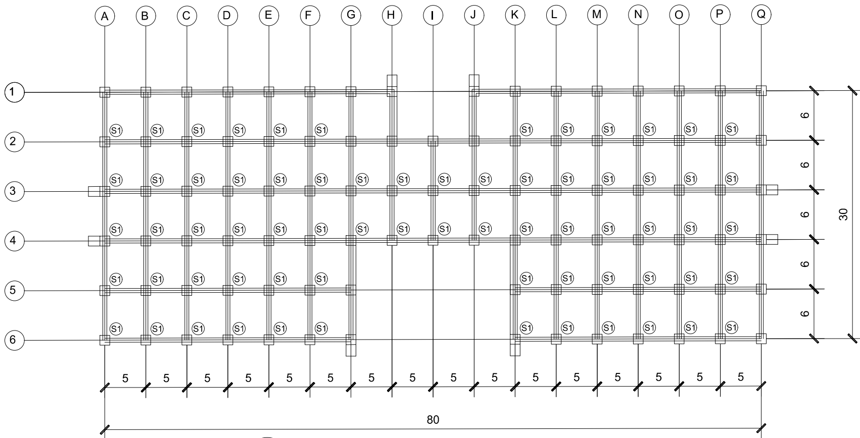
FIFTH FLOOR SLAB LAYOUT
