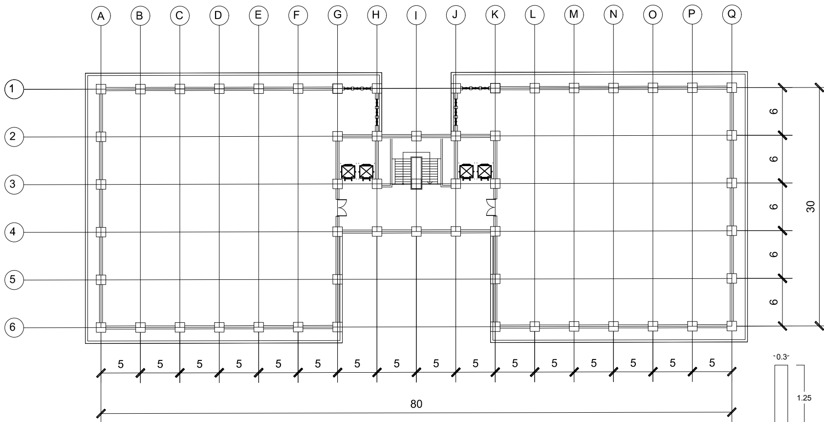
ROOF DECK PLAN
