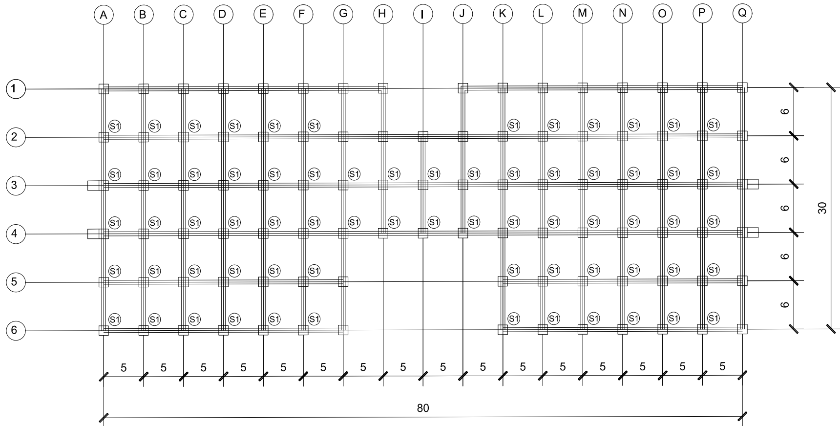
SECOND FLOOR SLAB LAYOUT
