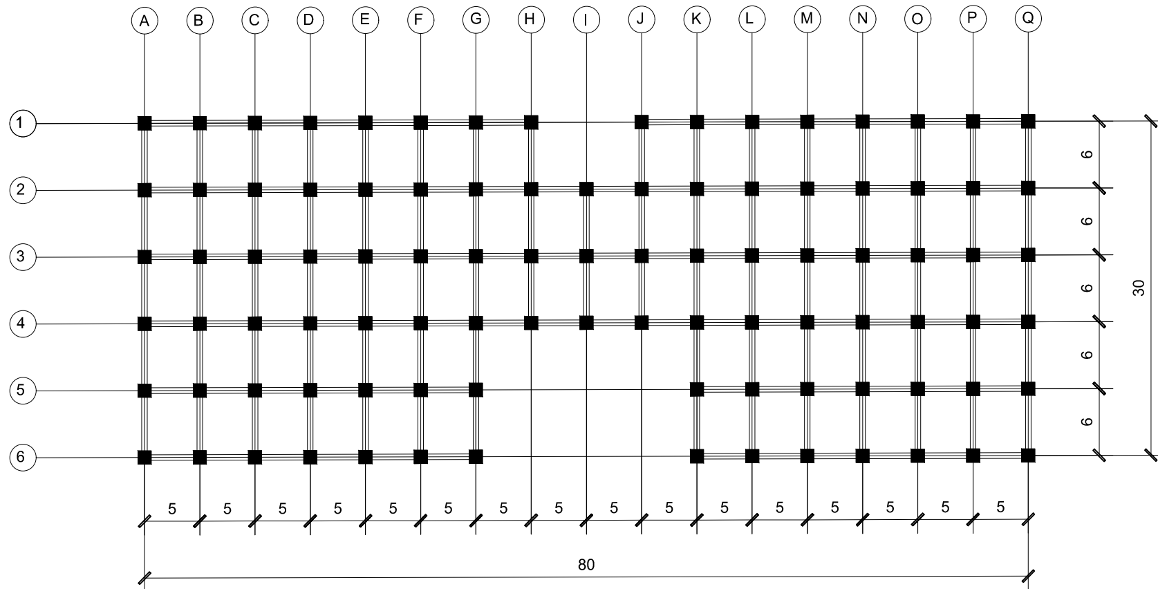
FIFTH FLOOR STRUCTURAL FRAME
