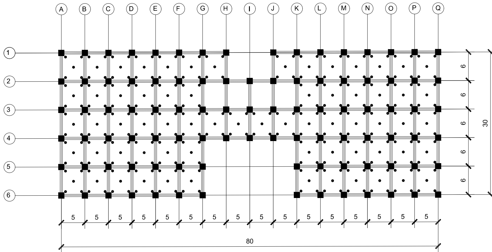
GROUND FLOOR CEILING PLAN 1:100
