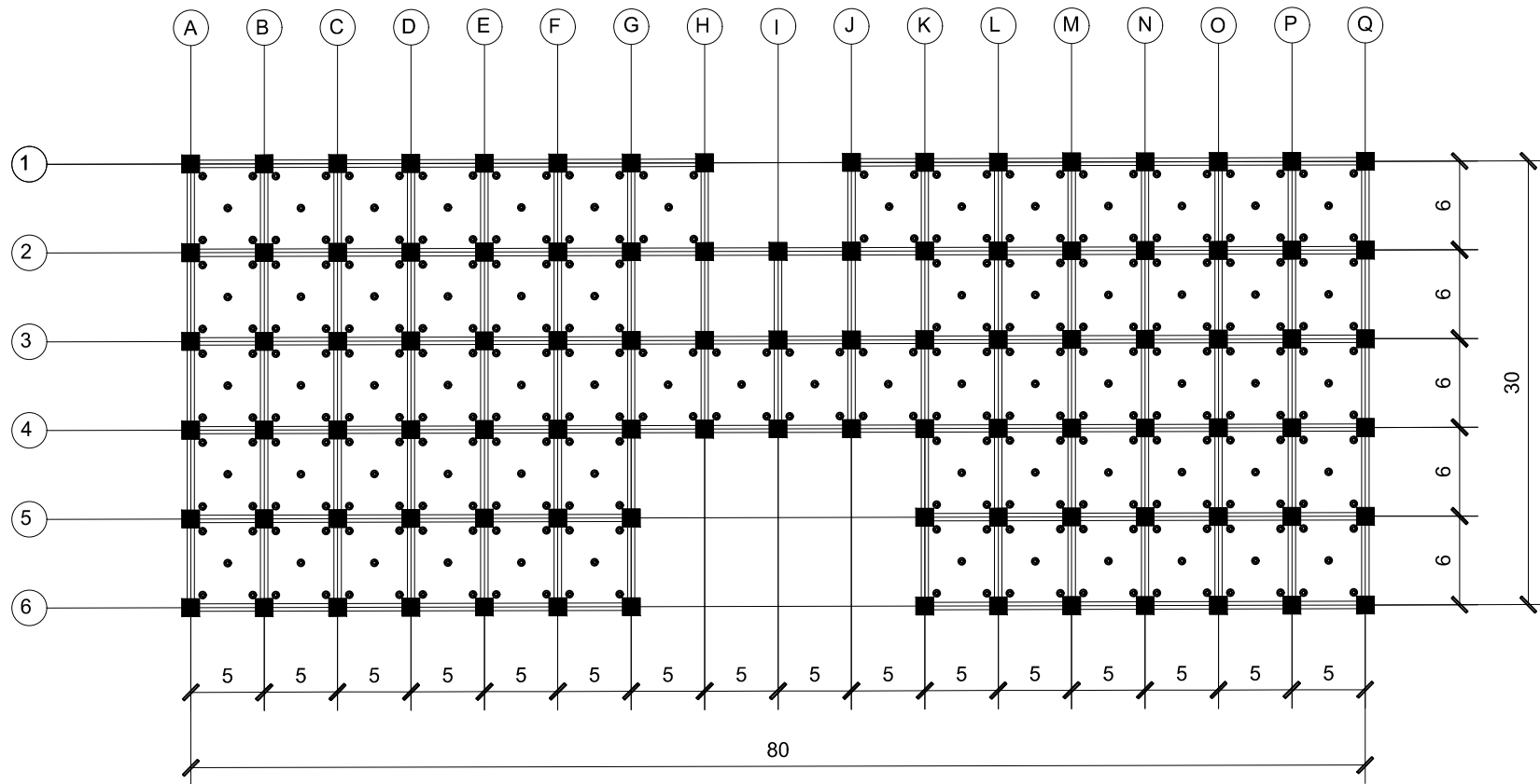
SIXTH FLOOR CEILING PLAN
