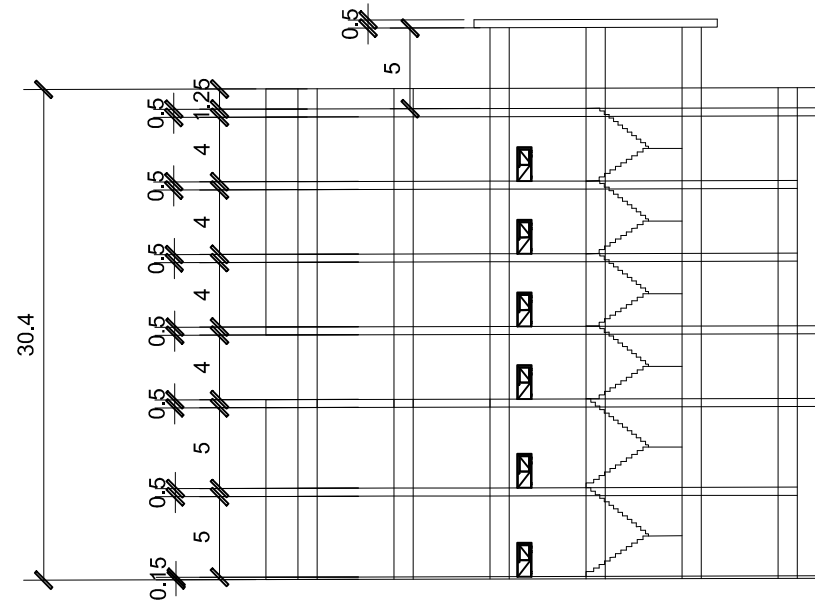
CROSS SECTION
