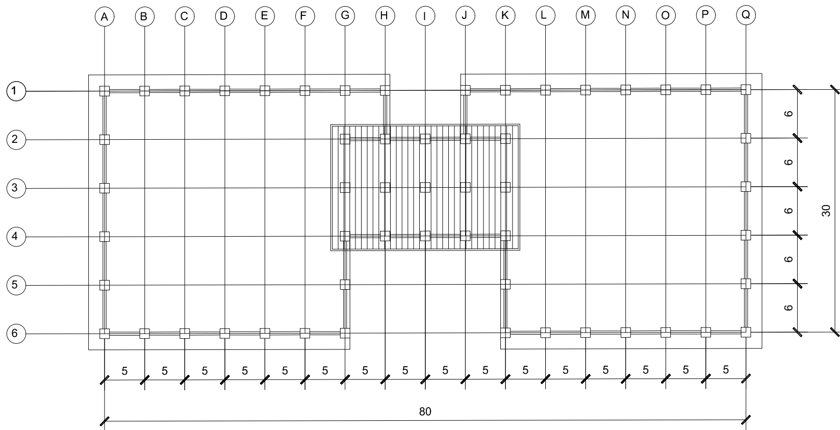
ROOF FRAMING PLAN 1:100
