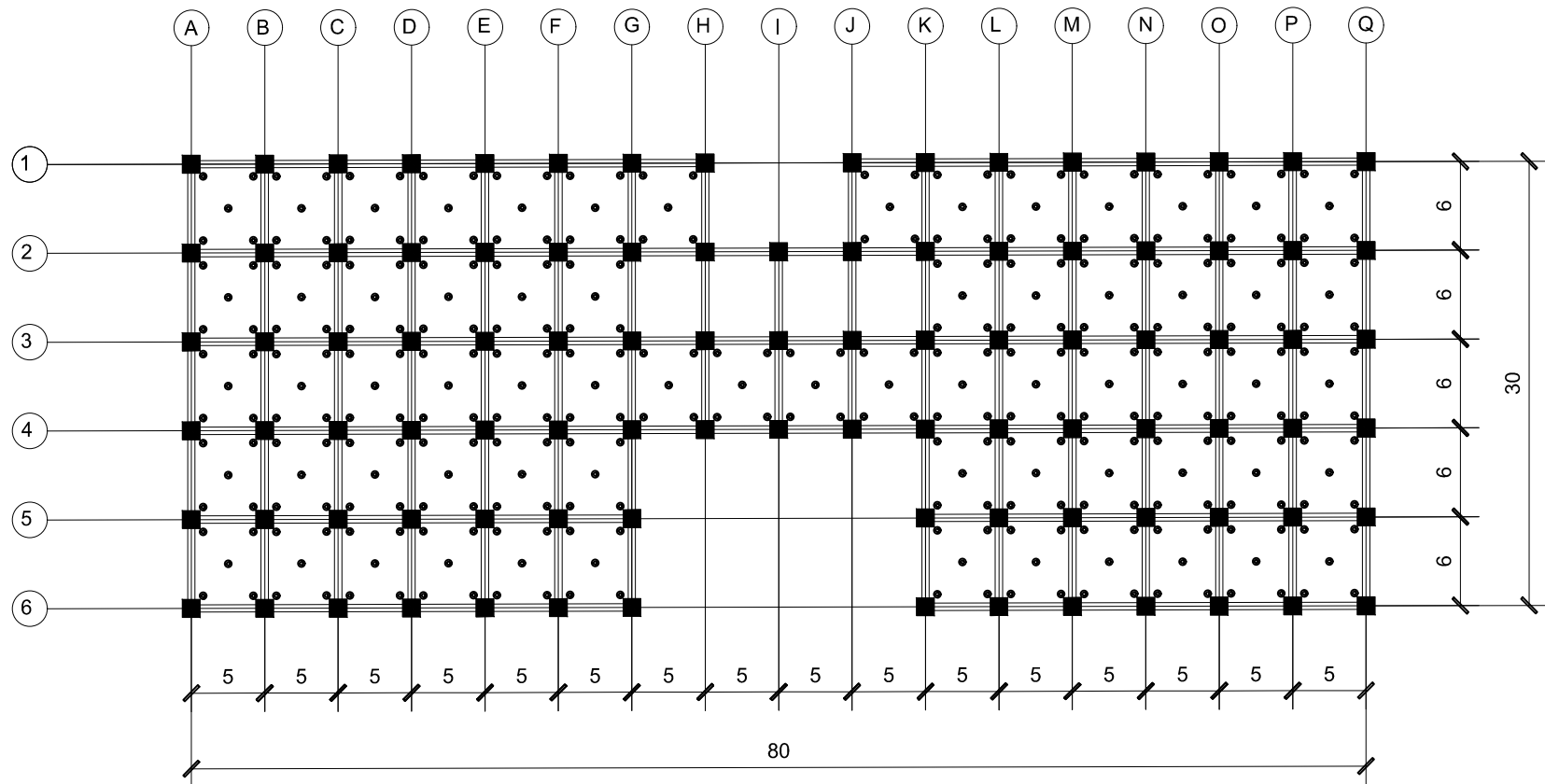
THIRD FLOOR CEILING PLAN
