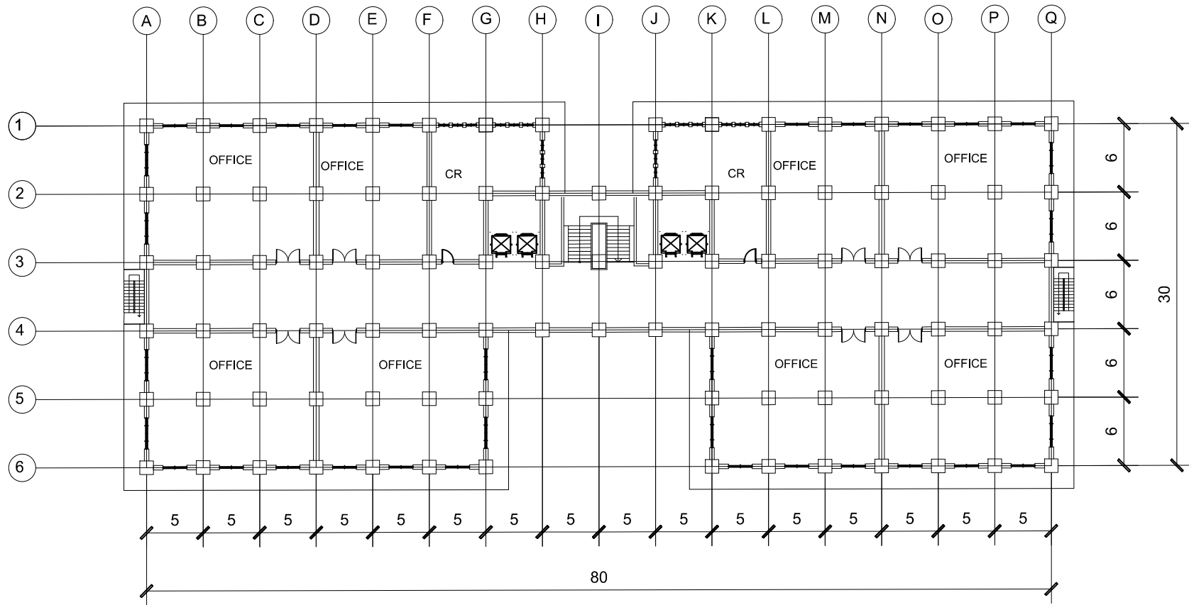
THIRD FLOOR PLAN 1:100
