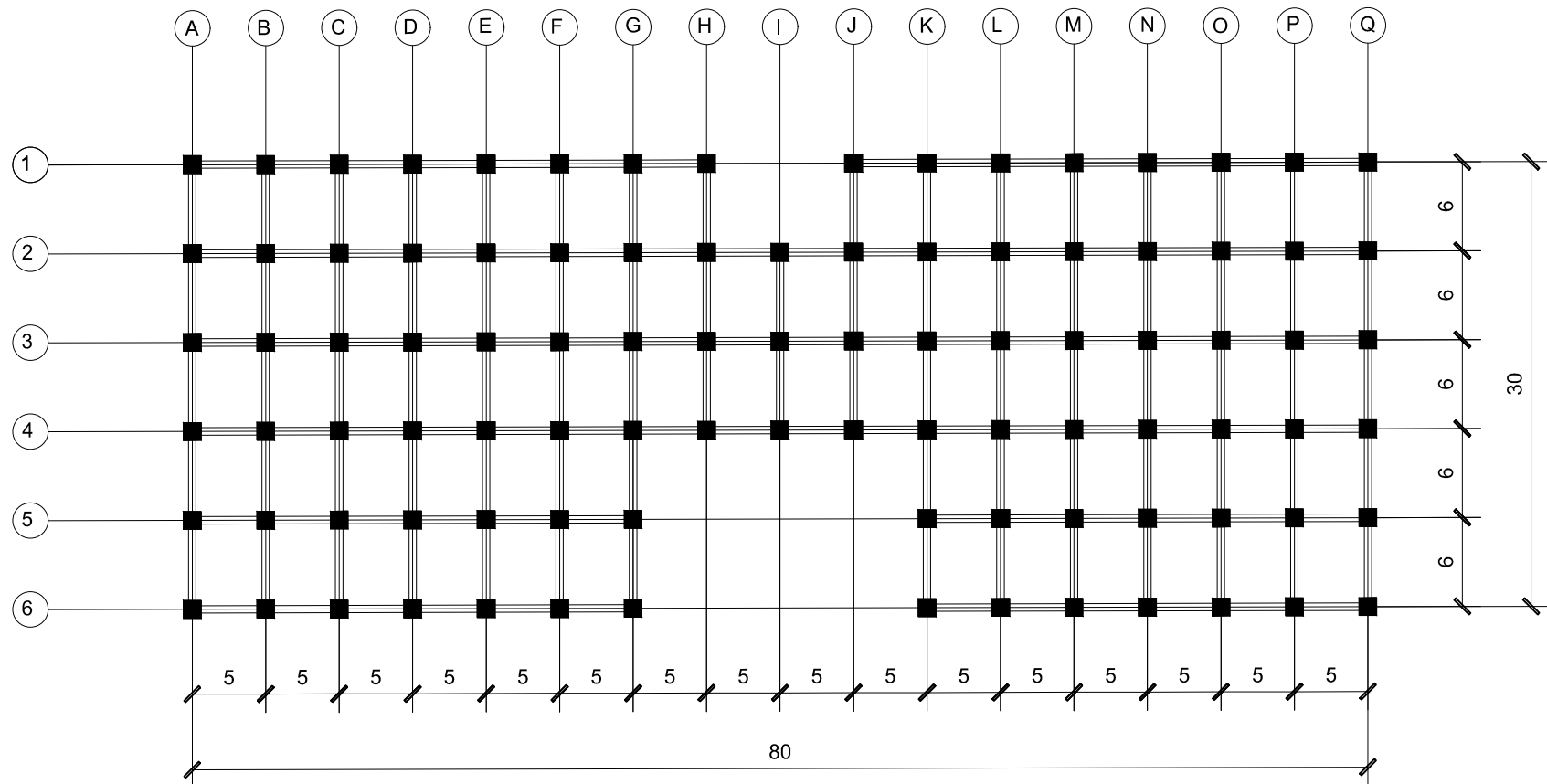
GROUND FLOOR STRUCTURAL FRAME
