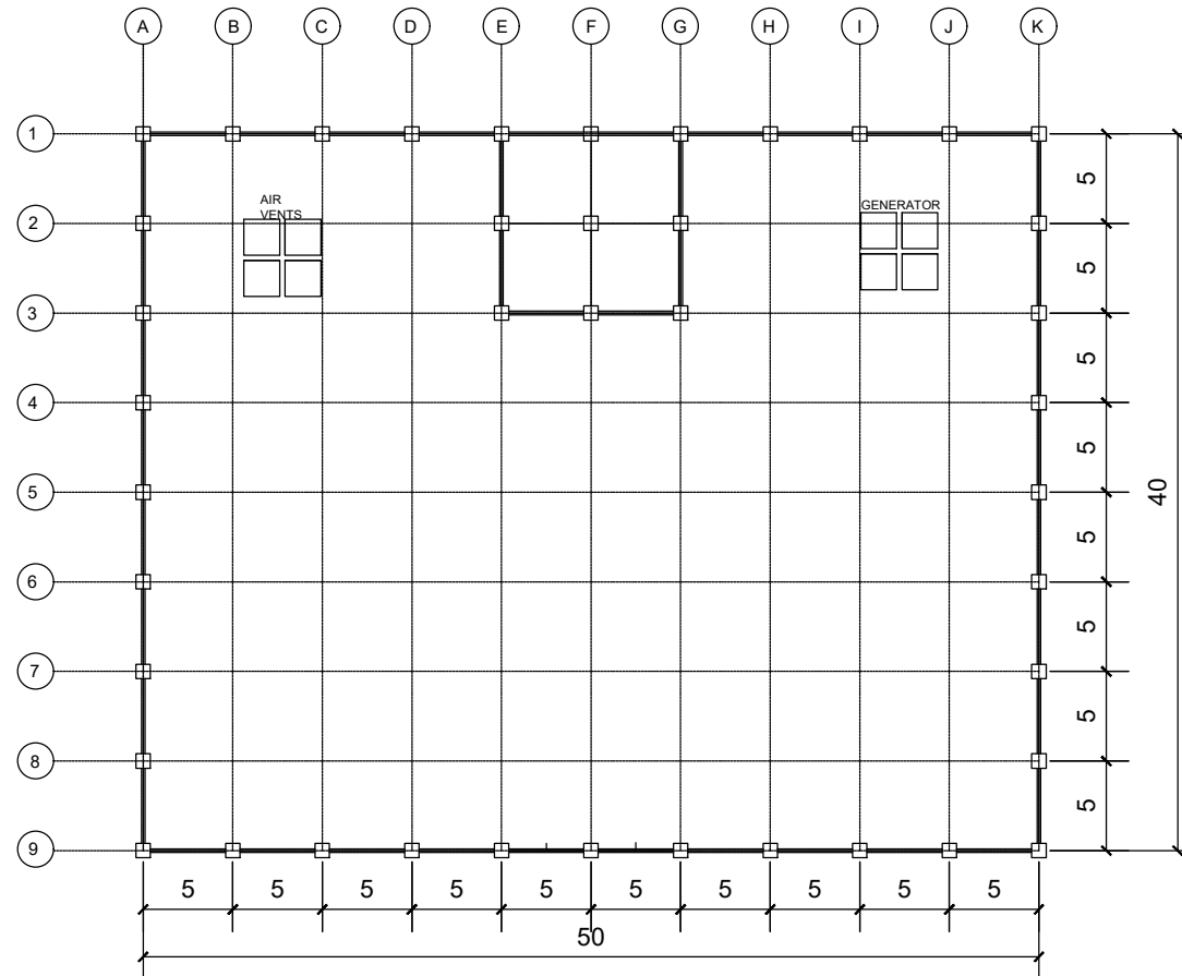
A-2 11 ROOFDECK FLOOR PLAN SCALE NTS
