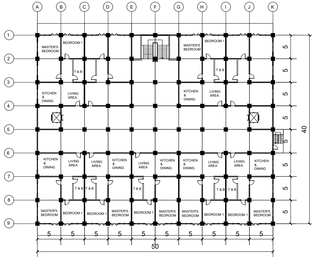
A-2 8 SCALE NTS FOURTH FLOOR PLAN
