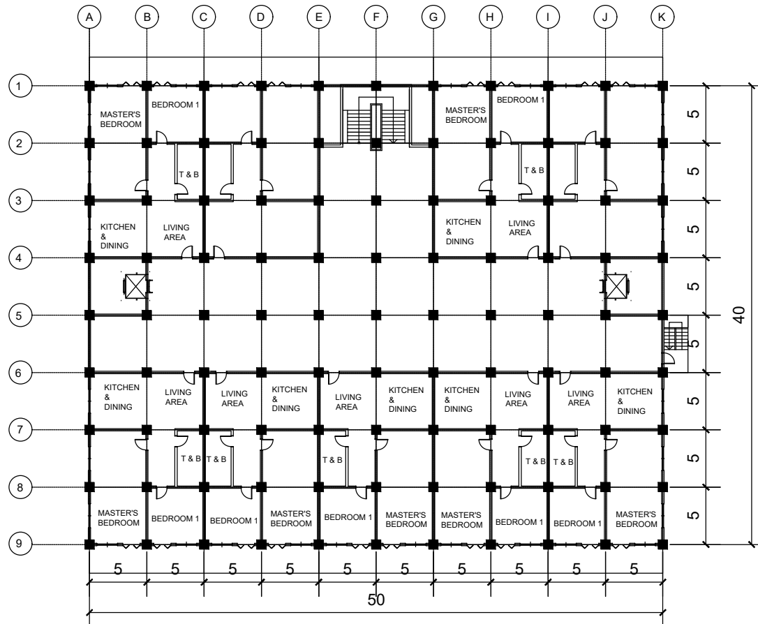
A-2 7 THIRD FLOOR PLAN SCALE _____ NTS
