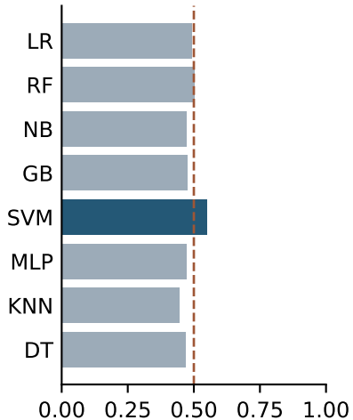
Balanced accuracy
