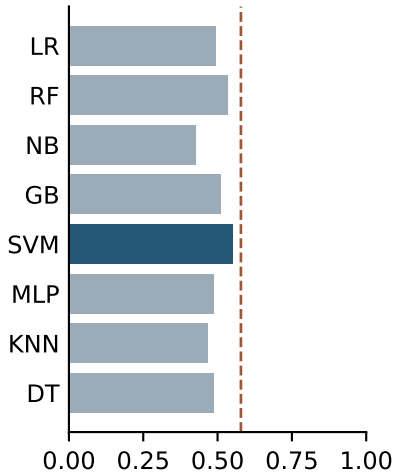
Accuracy
