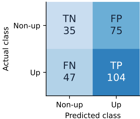
Held-out confusion matrix
