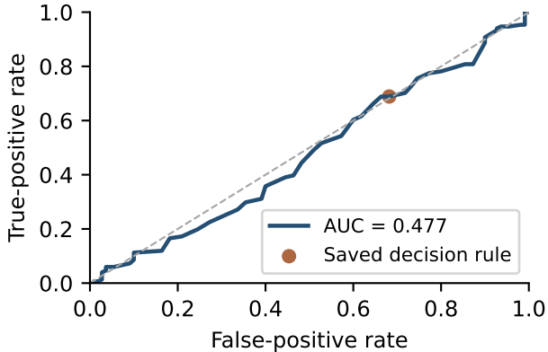
ROC from continuous scores
