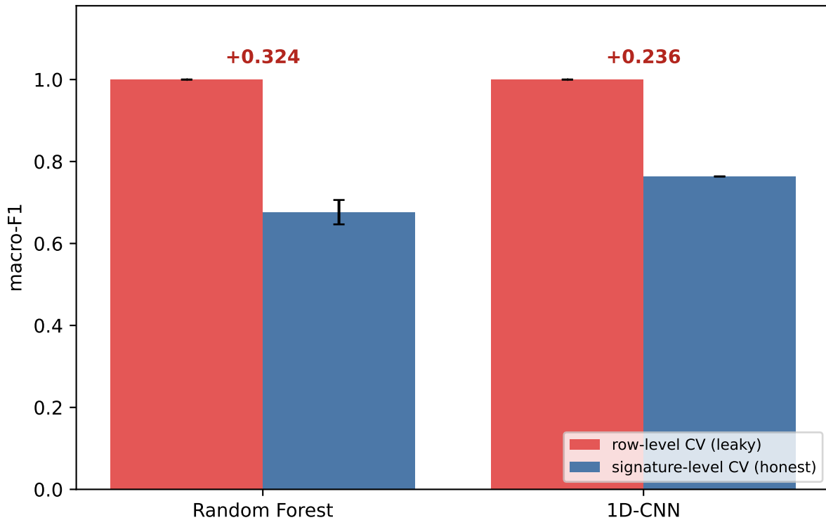
ciciov2024: the accuracy trap (99.7% duplicated rows) inflation = what a leaky evaluation invents
