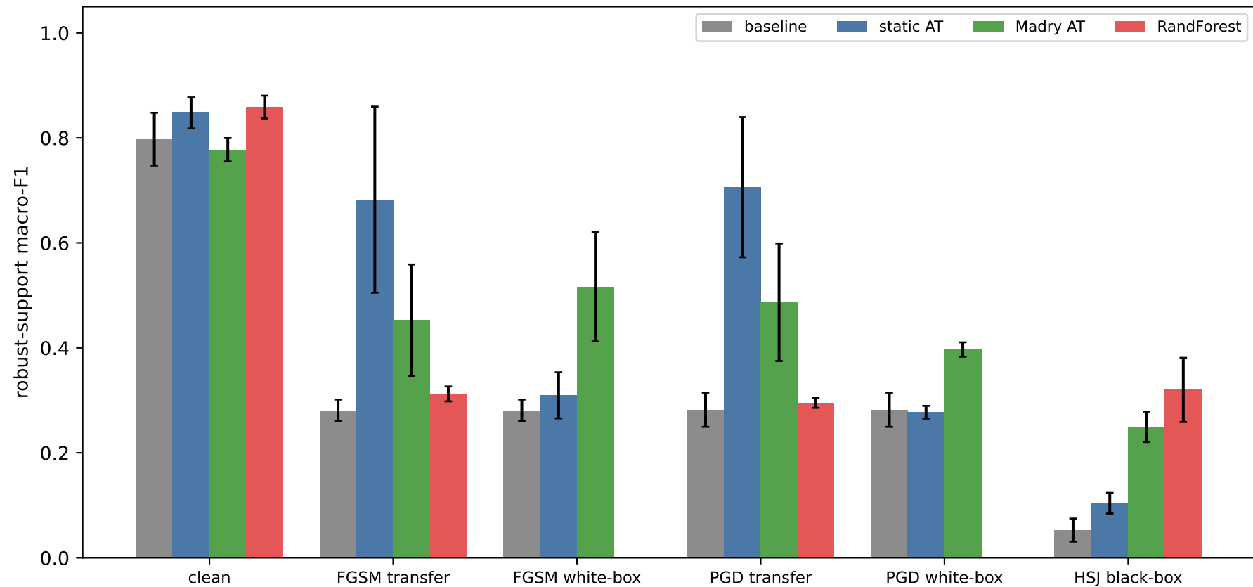
ciciov2024: attack x model grid (eps=0.1, mean \pm std over 5 repeats; hatched = subsample)
