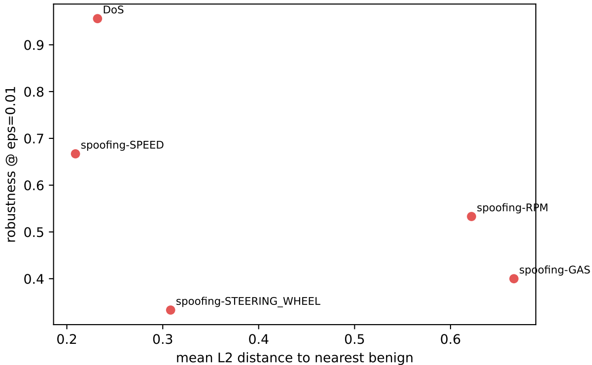
ciciov2024: robustness falls with distance (inverted) (exploratory, r=-0.531 , n=5 classes)
