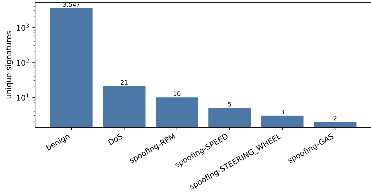
ciciov2024: attack-signature diversity
