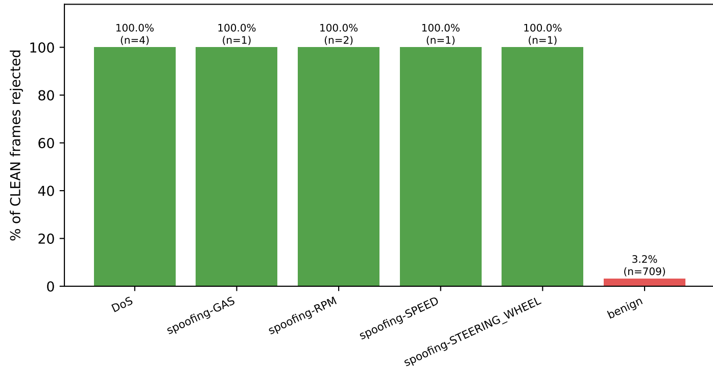
ciciov2024: envelope on unperturbed frames (green = attack recall, red = benign false alarms) as a standalone detector: precision 0.281, recall 1.000, F1 0.439
