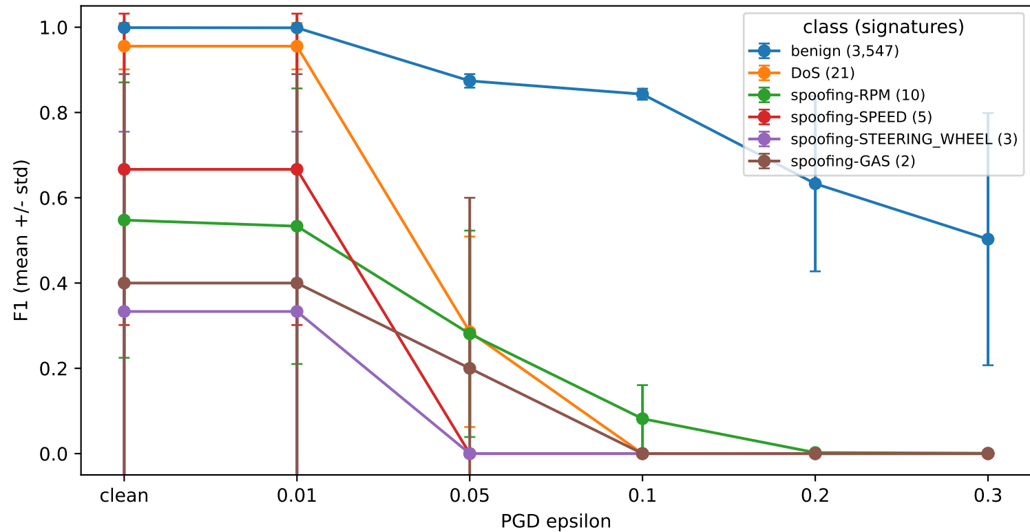
ciciov2024: per-class robustness under PGD
