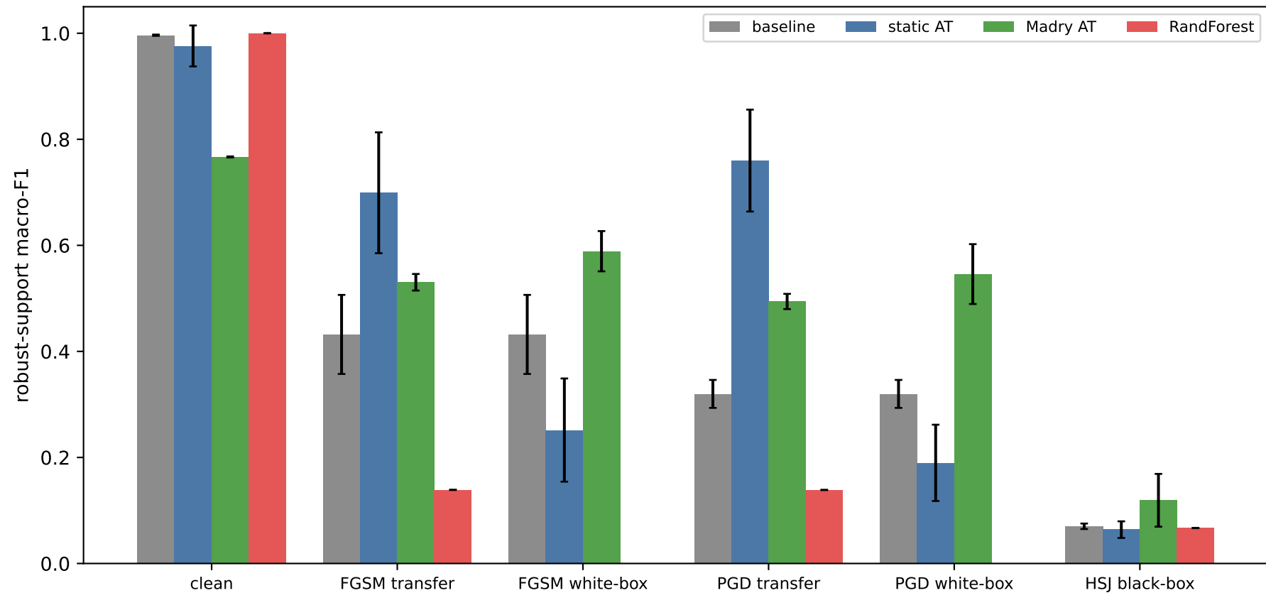
road: attack x model grid (eps=0.1, mean \pm std over 5 repeats; hatched = subsample)
