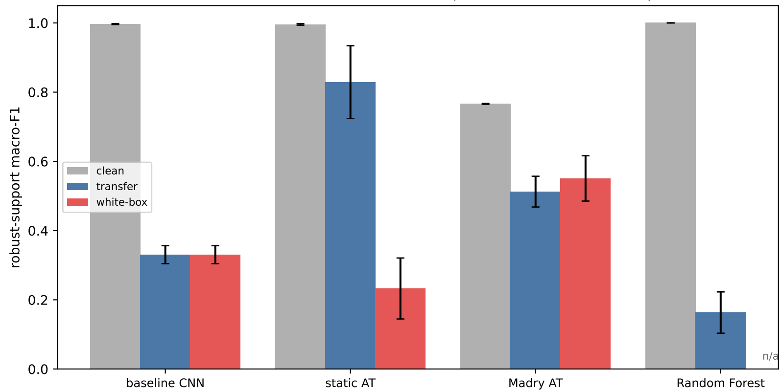
road: defence under two threat models (PGD eps=0.1, mean \pm std over 10 repeats)
