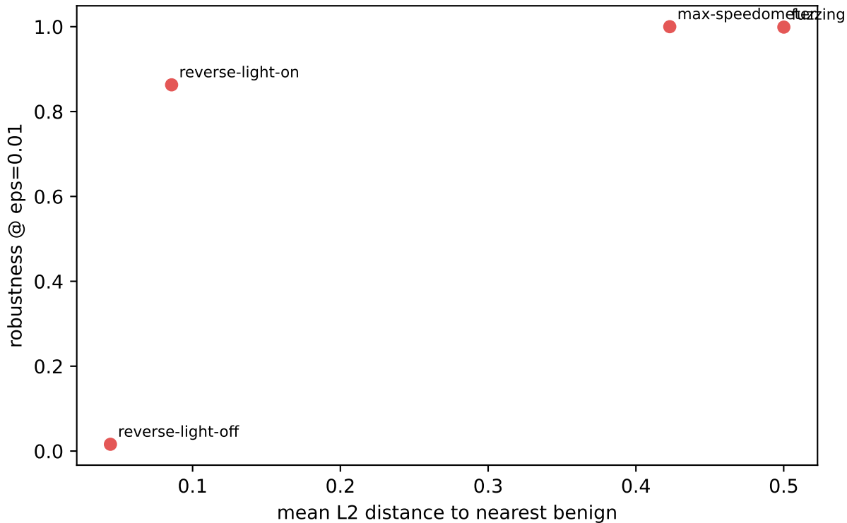
road: robustness rises with distance (exploratory, r=0.728 , n=4 classes)
