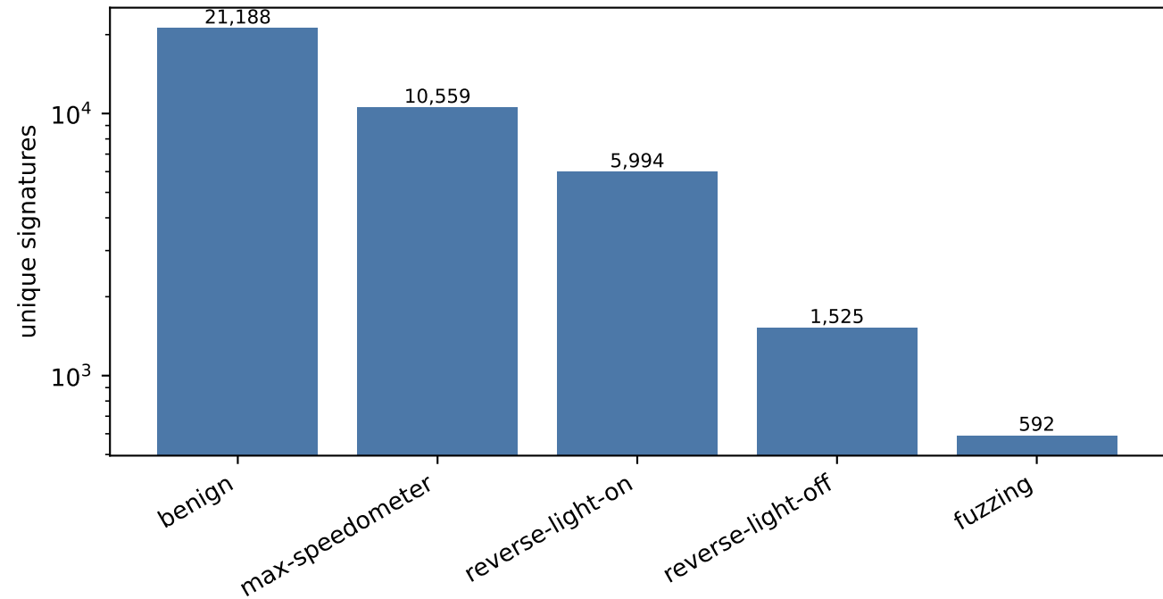
road: attack-signature diversity
