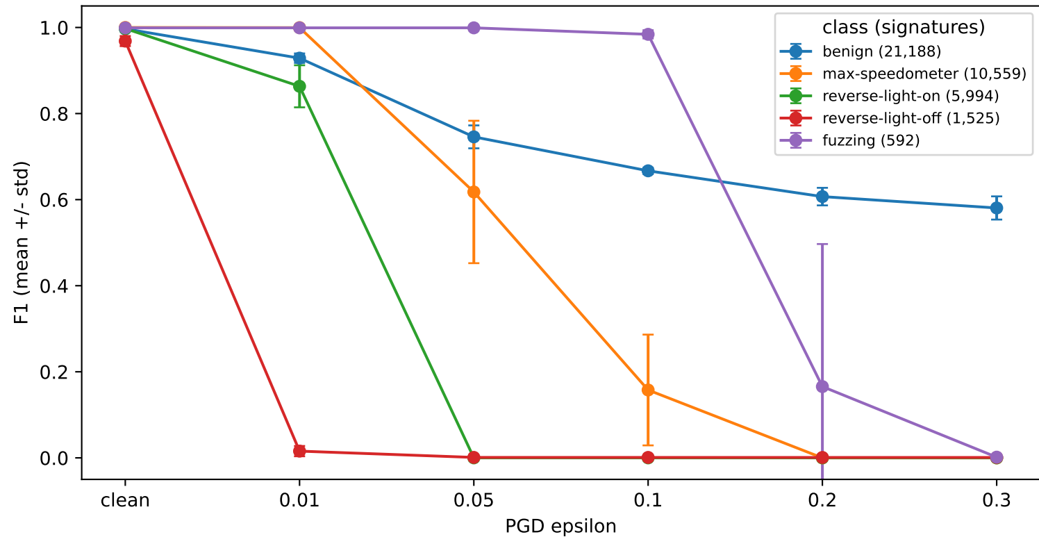
road: per-class robustness under PGD
